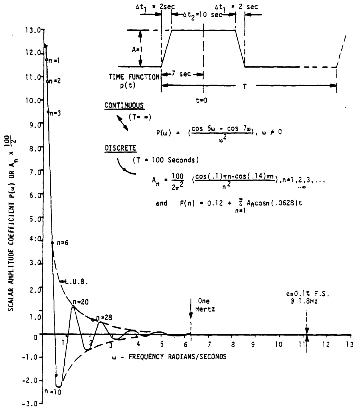
Figure 7. Frequency Spectrum-Facility Induced Pressure Transient
