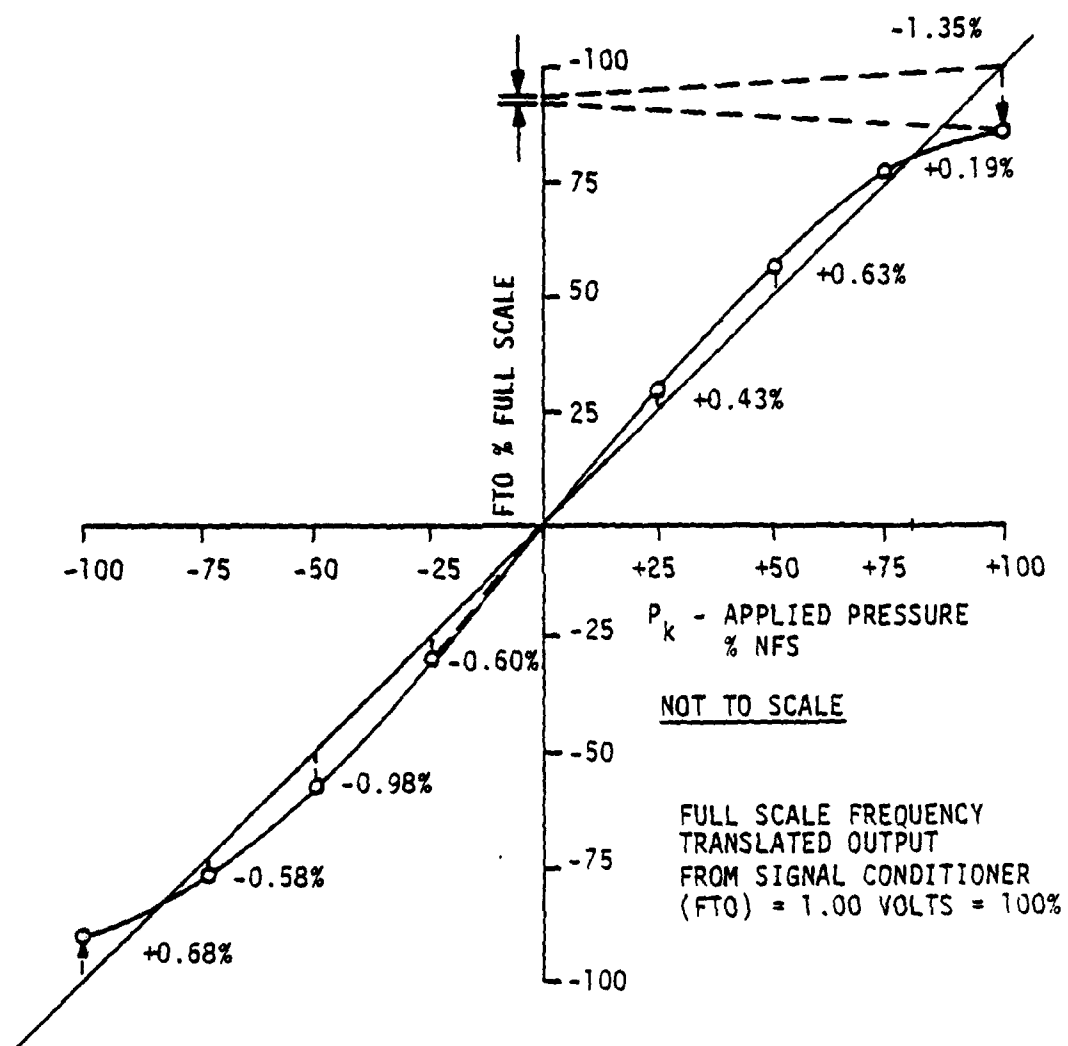
Figure 62. Installed System Pre-Test Calibration Data - Transducer A-18
