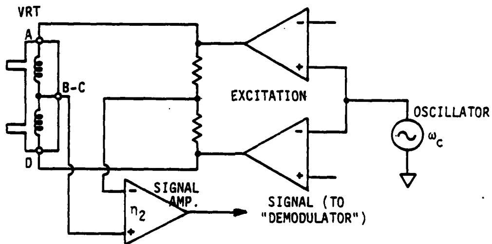
Figure E-1. Transducer Applications Circuitry
