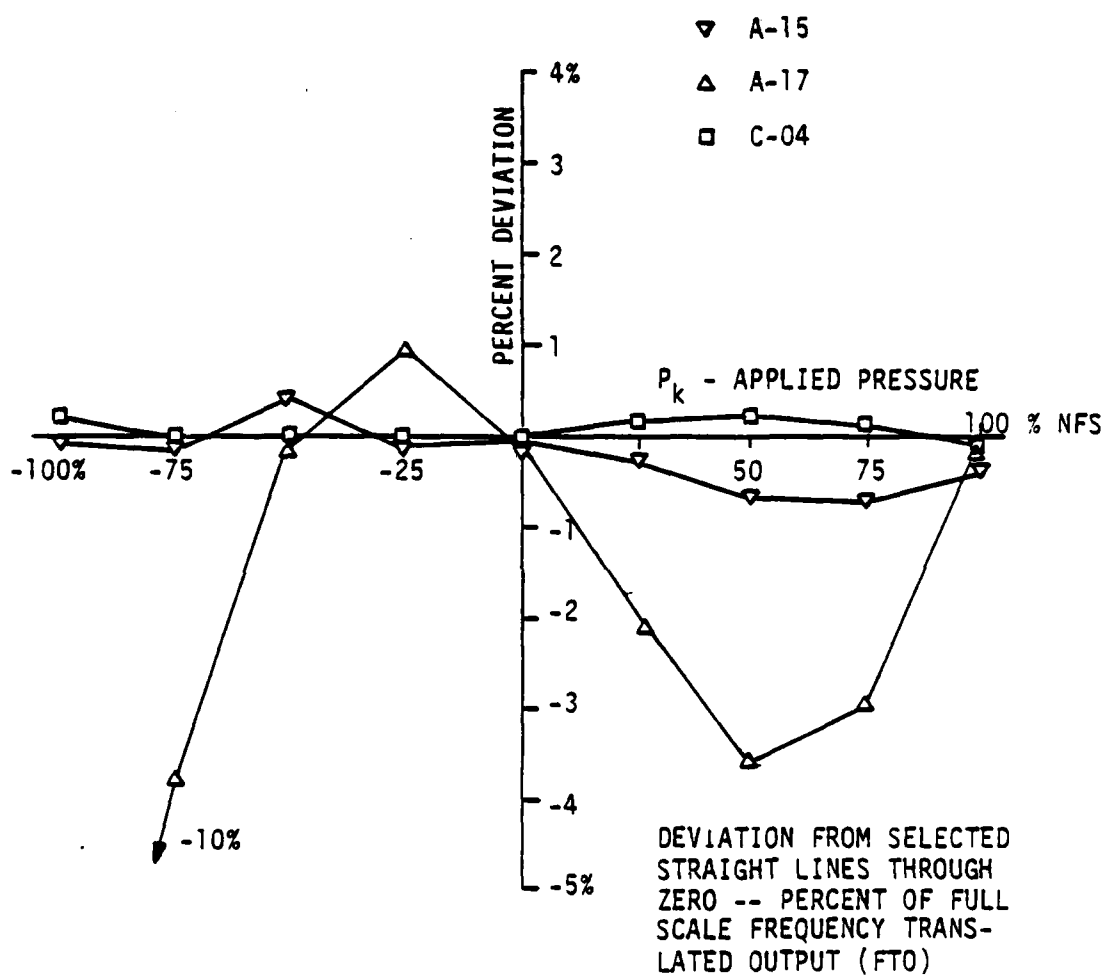
Figure 60. Installed System Pre-Test Calibration Data - Transducers A-15, A-17, and C-04
