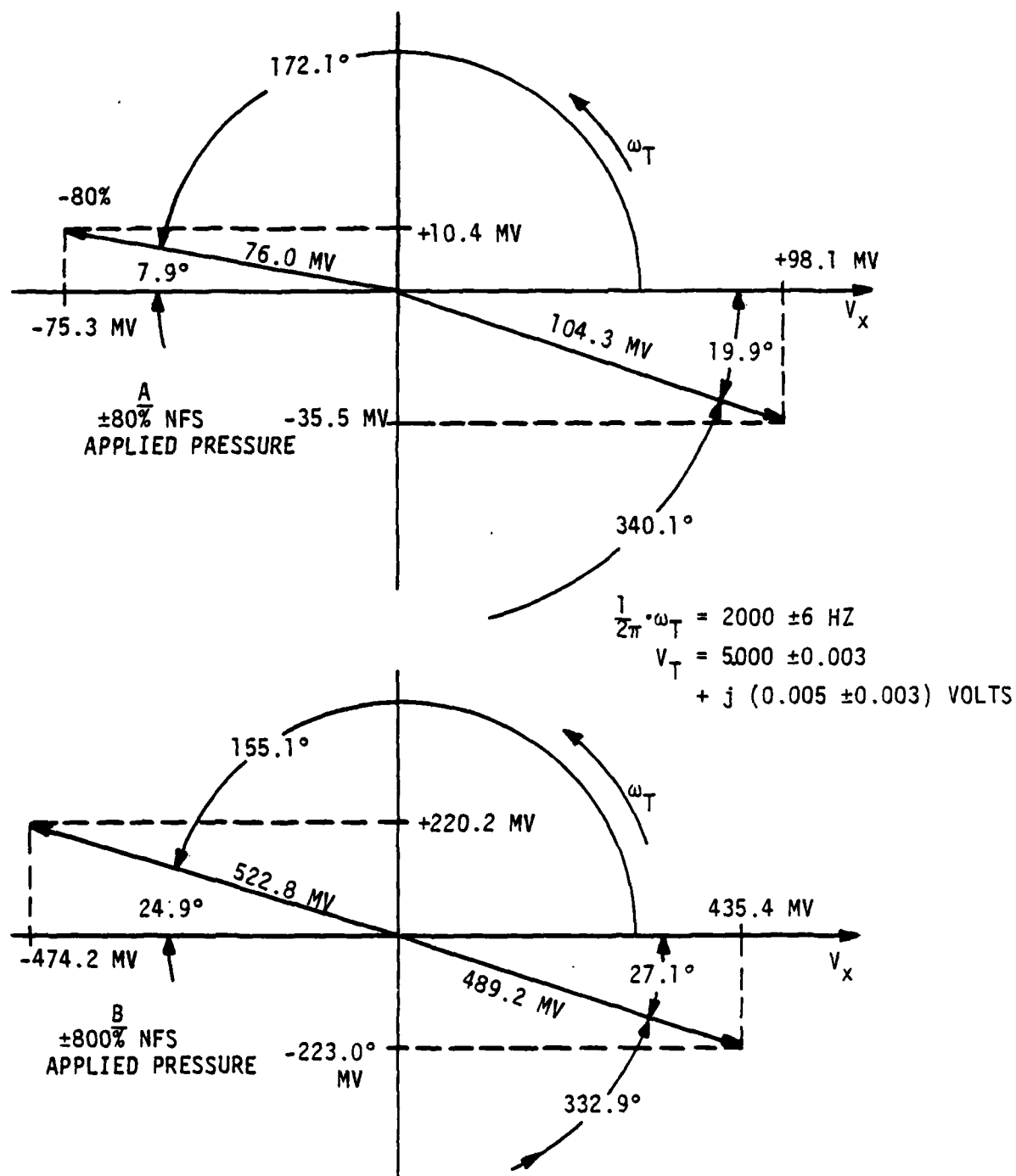
Figure 65. Fundamental Frequency Signal Phasors - Applied Pressure P_k = \pm 80\% and \pm 800\% \text{ NFS} - Transducer A-10
