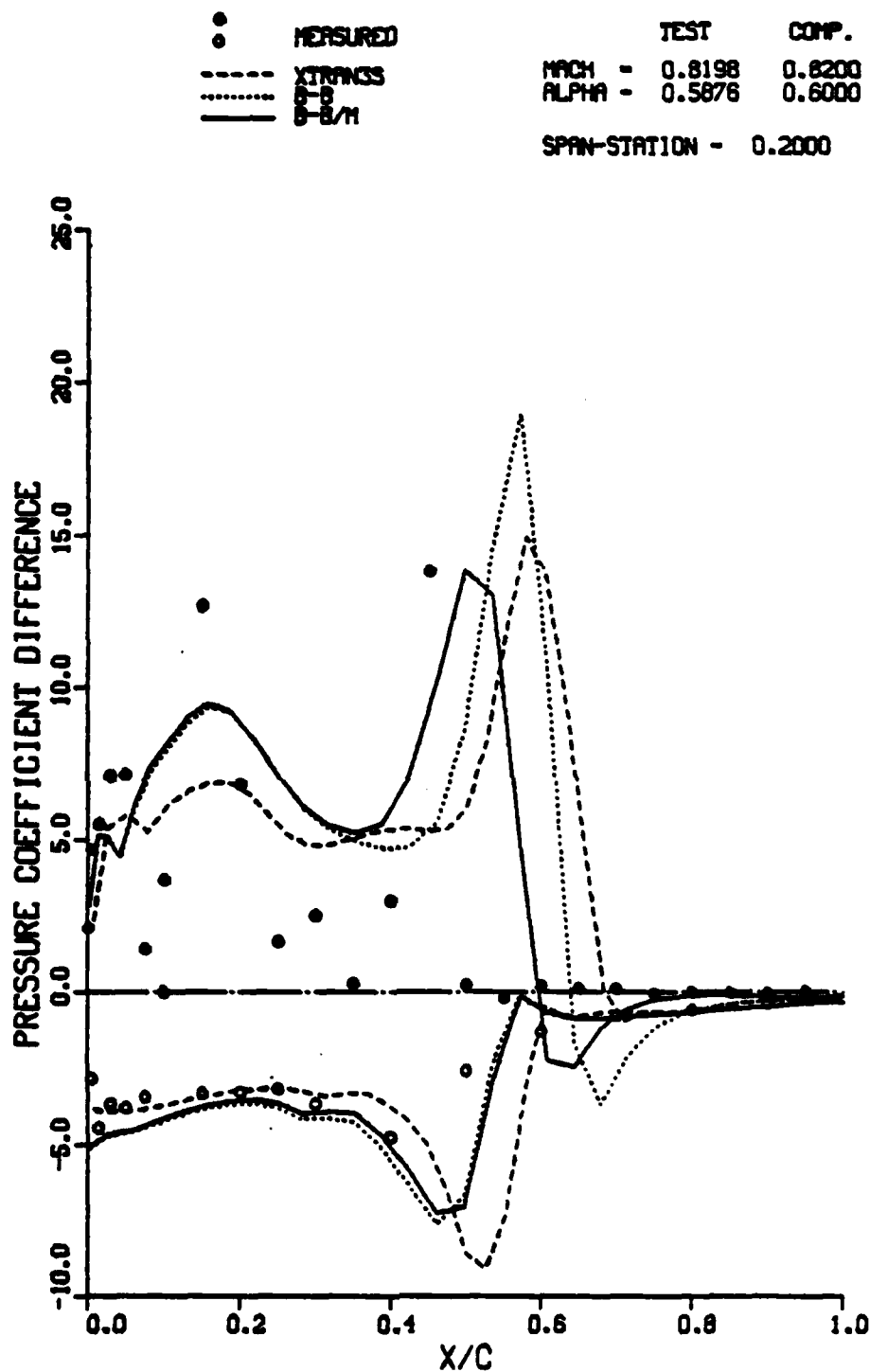
Figure 31. Comparison of Computed and Measured Quasi-Steady Pressure Difference at Several Span-Stations (Sheet 1 of 6)
