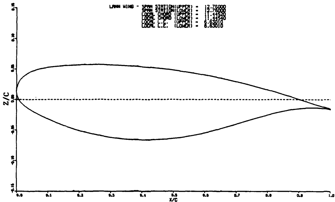
(c) SPAN-STATION = 0.32
