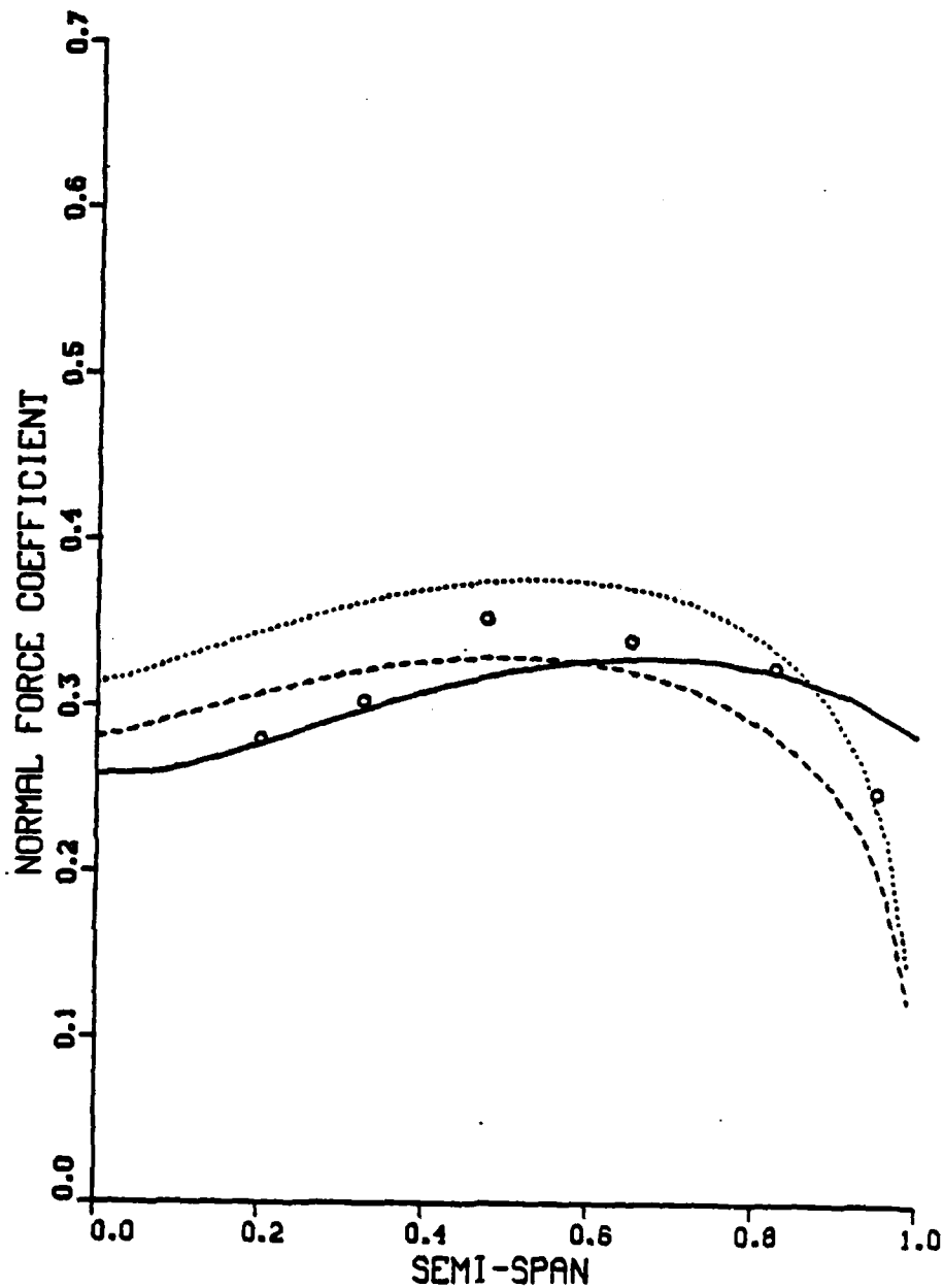
Figure 26. Comparison of Computed and Measured Span-Loading Distributions at Design Mach Number (Sheet 2 of 5)
