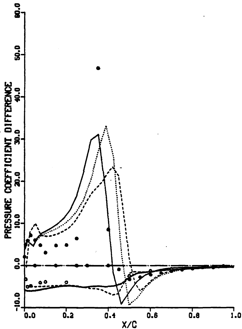
Figure 31. Comparison of Computed and Measured Quasi-Steady Pressure Difference at Several Span-Stations (Sheet 3 of 6)
