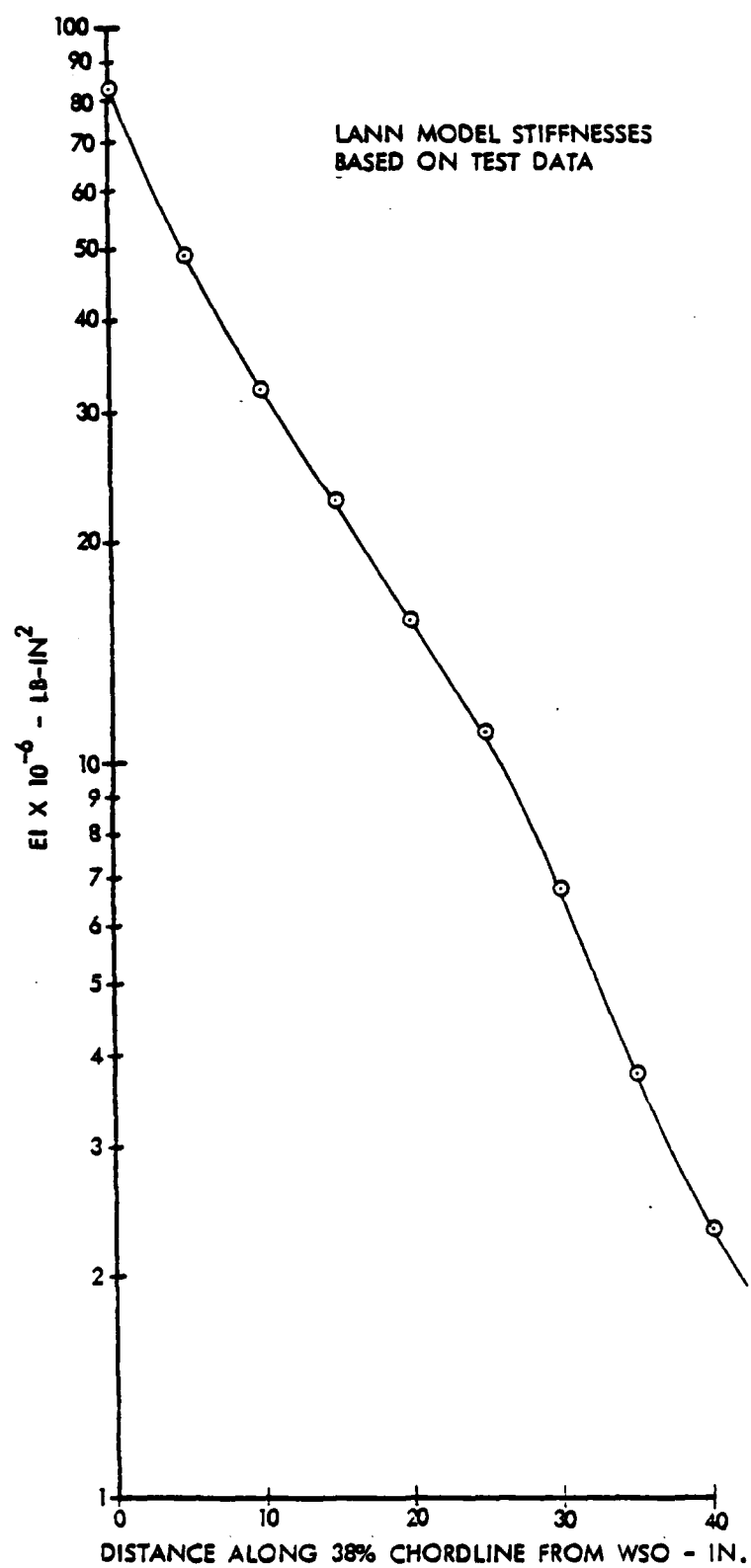
Figure 6. Bending Stiffness Distribution
