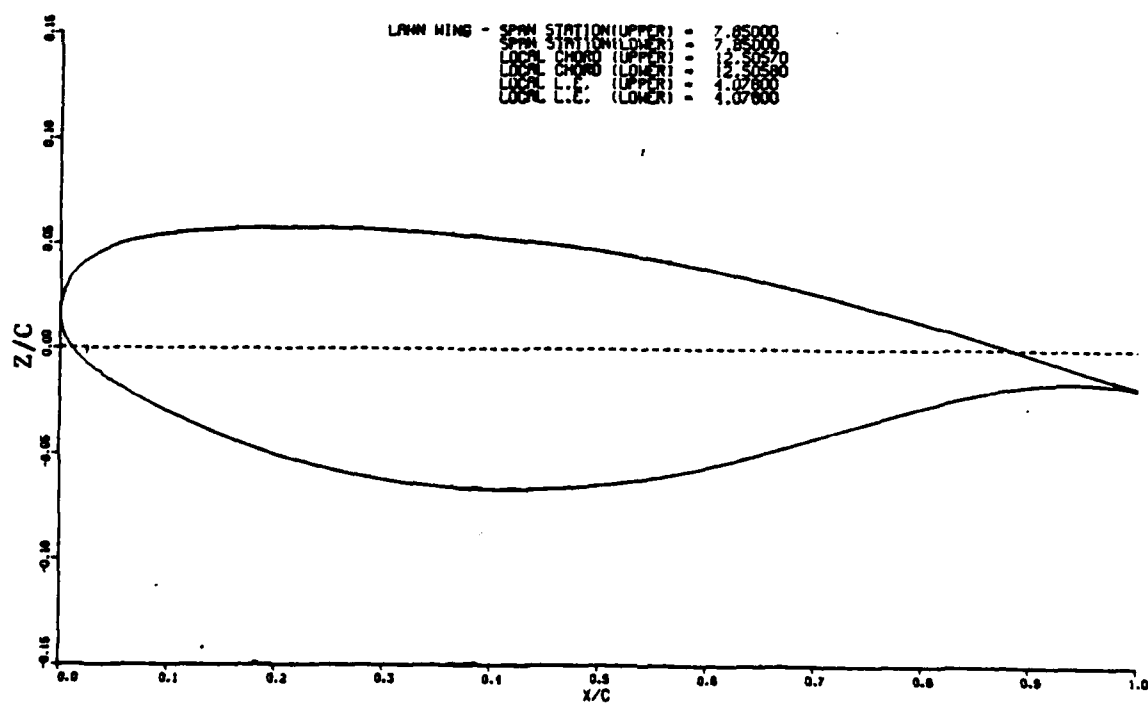
(b) SPAN-STATION = 0.20
