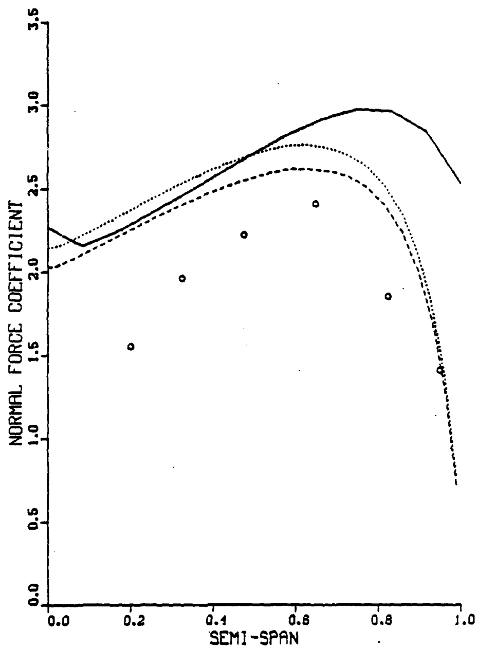
Figure 32. Comparison of Computed and Measured Quasi-Steady Span-Loading
