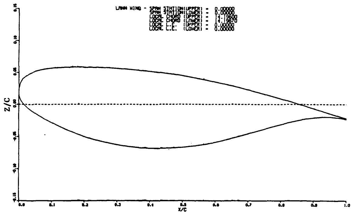
(a) SPAN-STATION = 0.00
