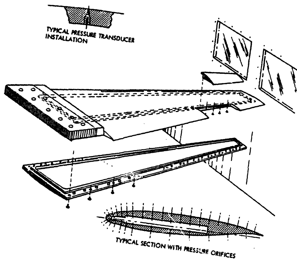
Figure 2. LANN Wing Assembly
