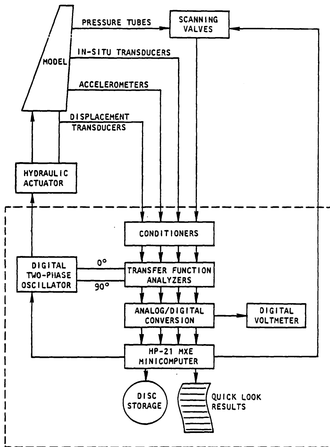
Figure 11. Block-Diagram of PHAROS Data Acquisition and Reduction System
