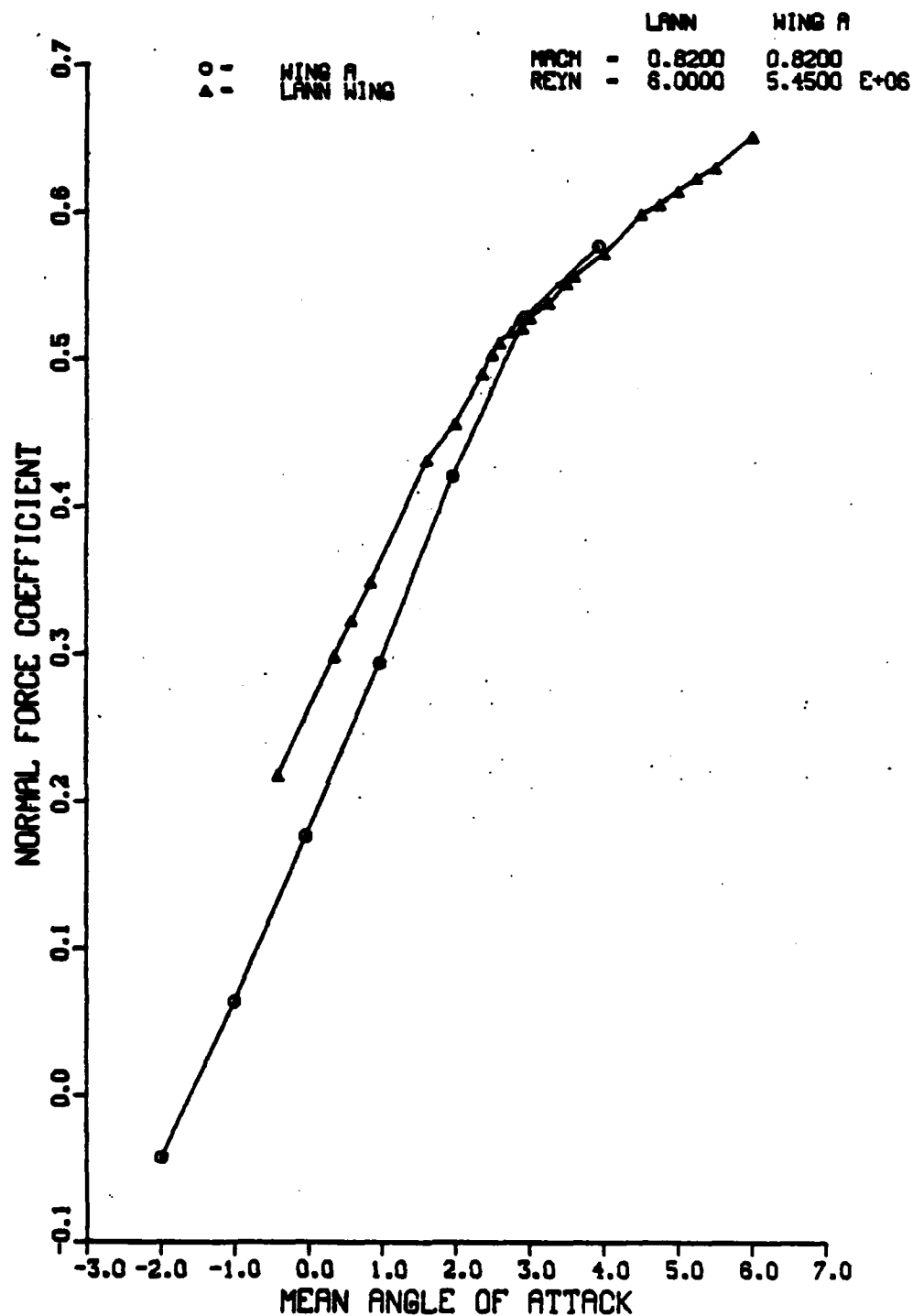
(a) MEASURED NORMAL FORCE OF LANN WING AND WING A
