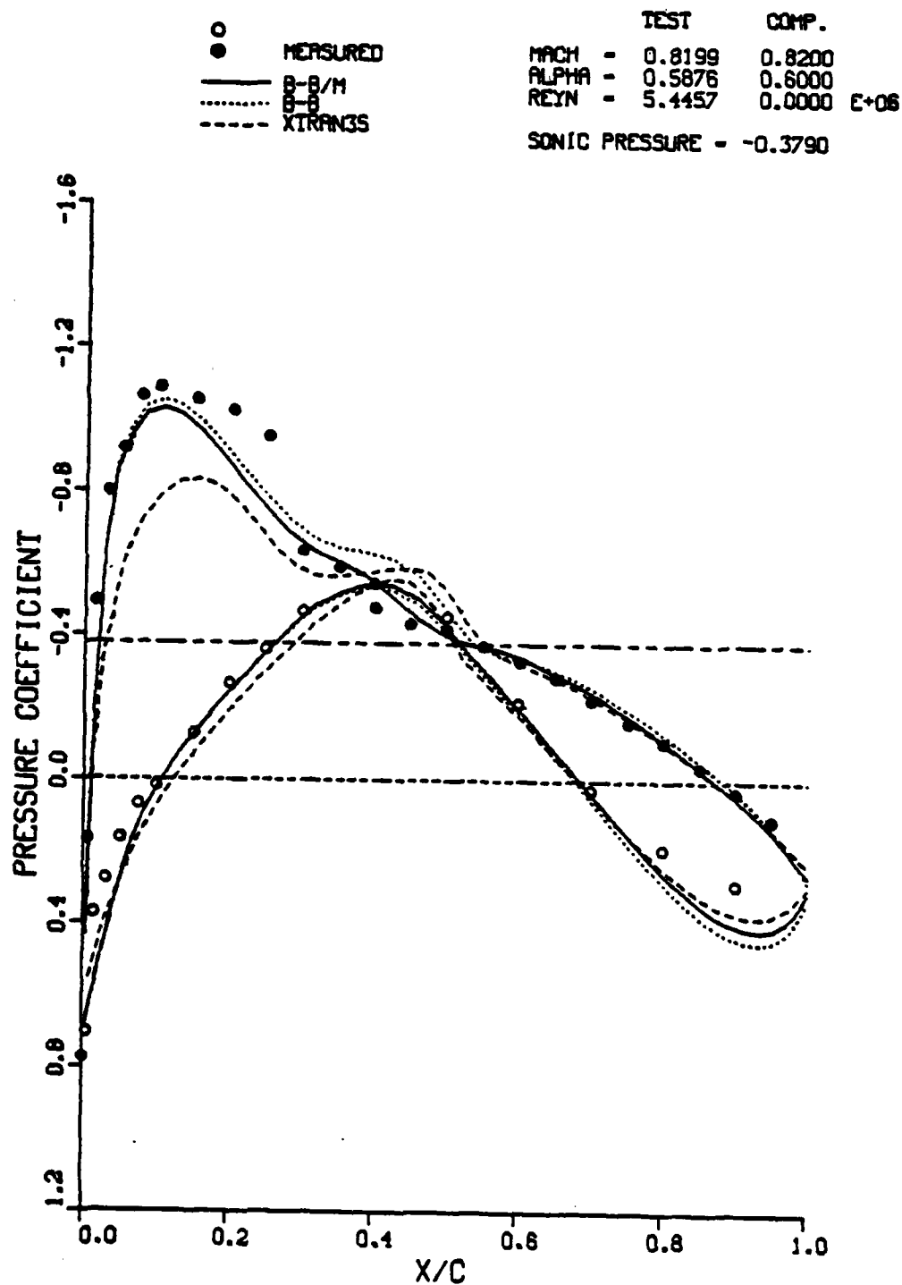
Figure 19. Comparison of Computed and Measured Pressure Distributions (Sheet 2 of 6)
