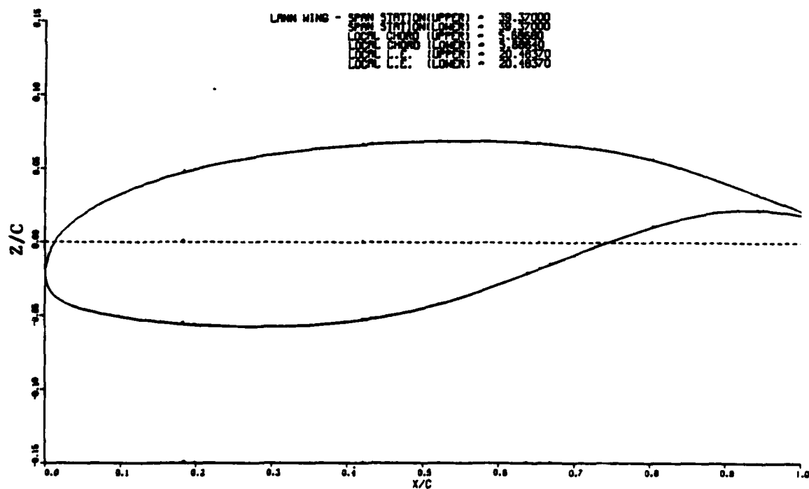
(h) SPAN-STATION = 1.00
