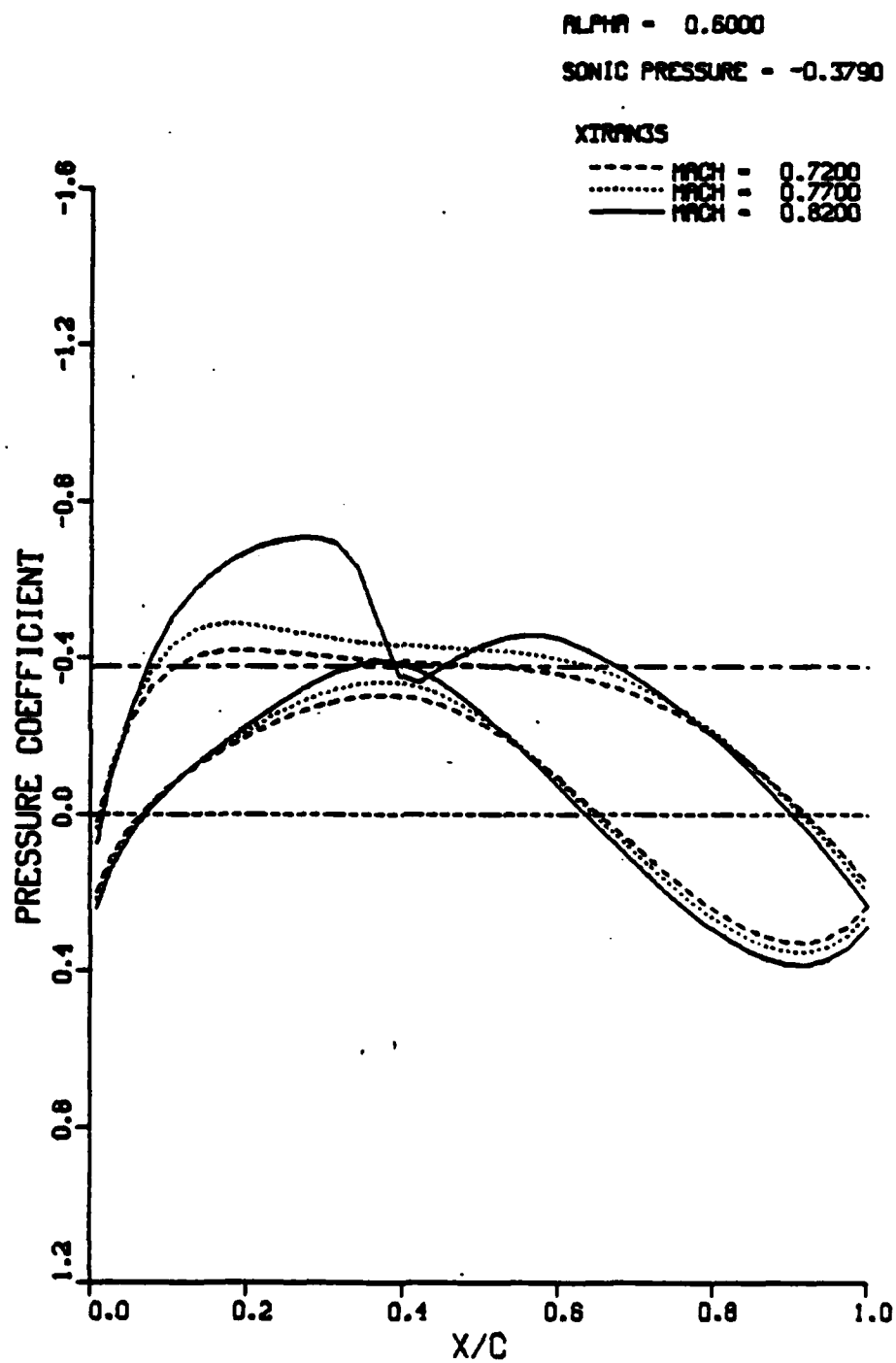
Figure 27. Effect of Mach Number Variation on Pressure Distributions for Fixed Mean Angle of Attack (Sheet 6 of 6)
