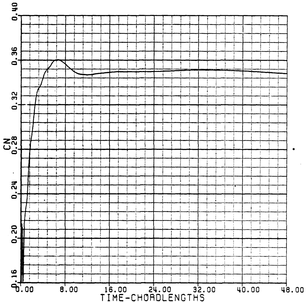
Figure 16. Time History of Steady Flow Calculations with XTRAN3S Code (Sheet 2 of 4)
