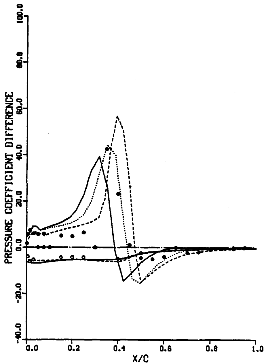
Figure 31. Comparison of Computed and Measured Quasi-Steady Pressure Difference at Several Span-Stations (Sheet 4 of 6)
