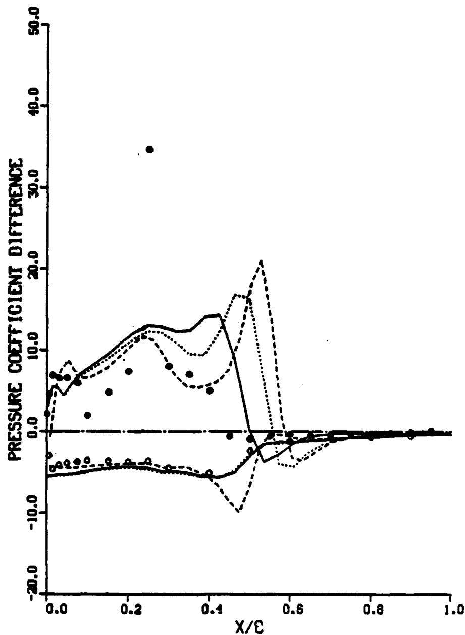
Figure 31. Comparison of Computed and Measured Quasi-Steady Pressure Difference at Several Span-Stations (Sheet 2 of 6)
