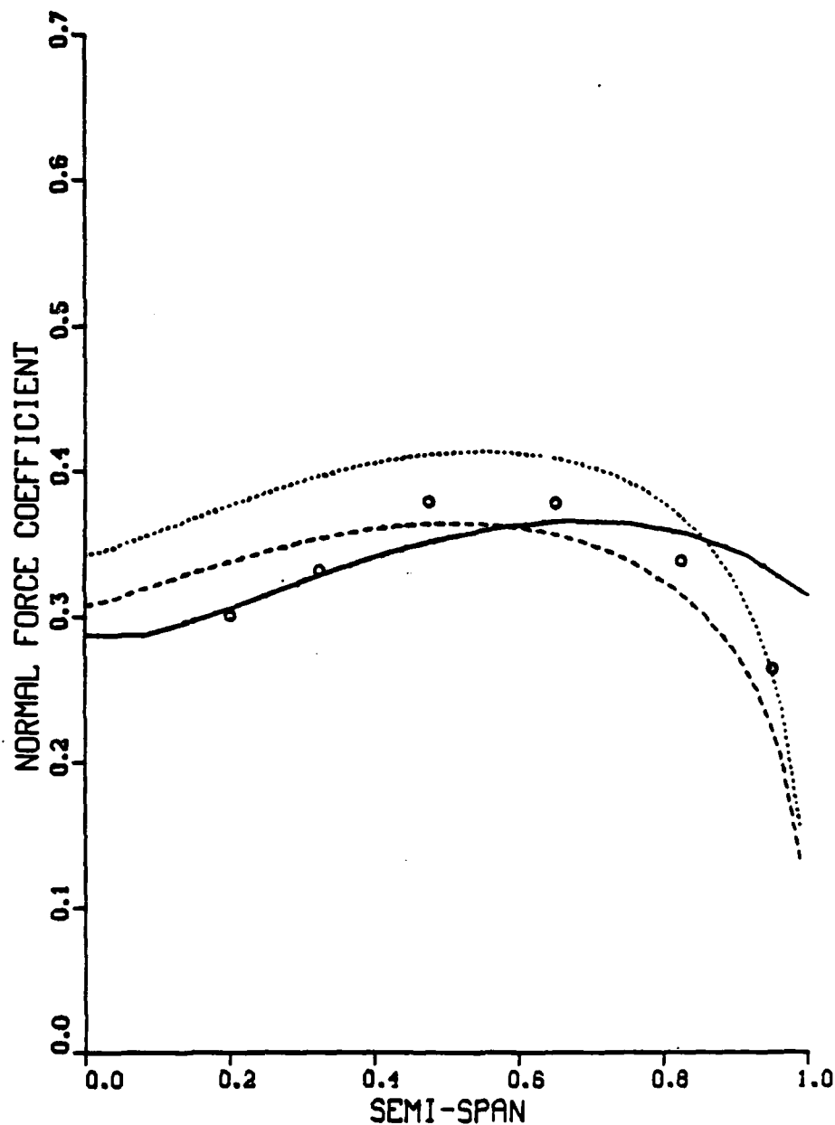
Figure 26. Comparison of Computed and Measured Span-Loading Distributions at Design Mach Number (Sheet 3 of 5)
