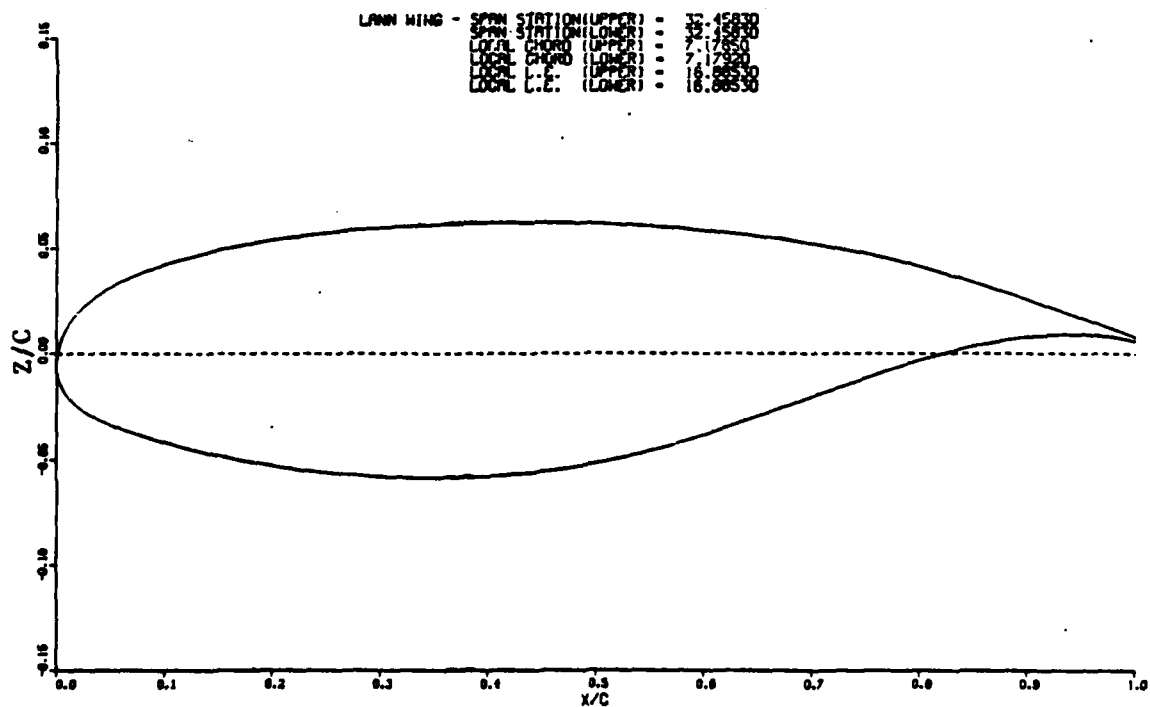
(f) SPAN-STATION = 0.82
