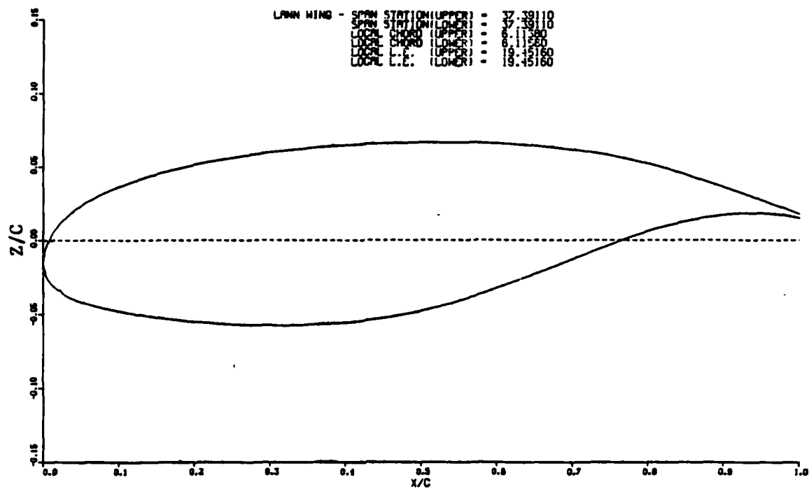
(g) SPAN-STATION = 0.95
