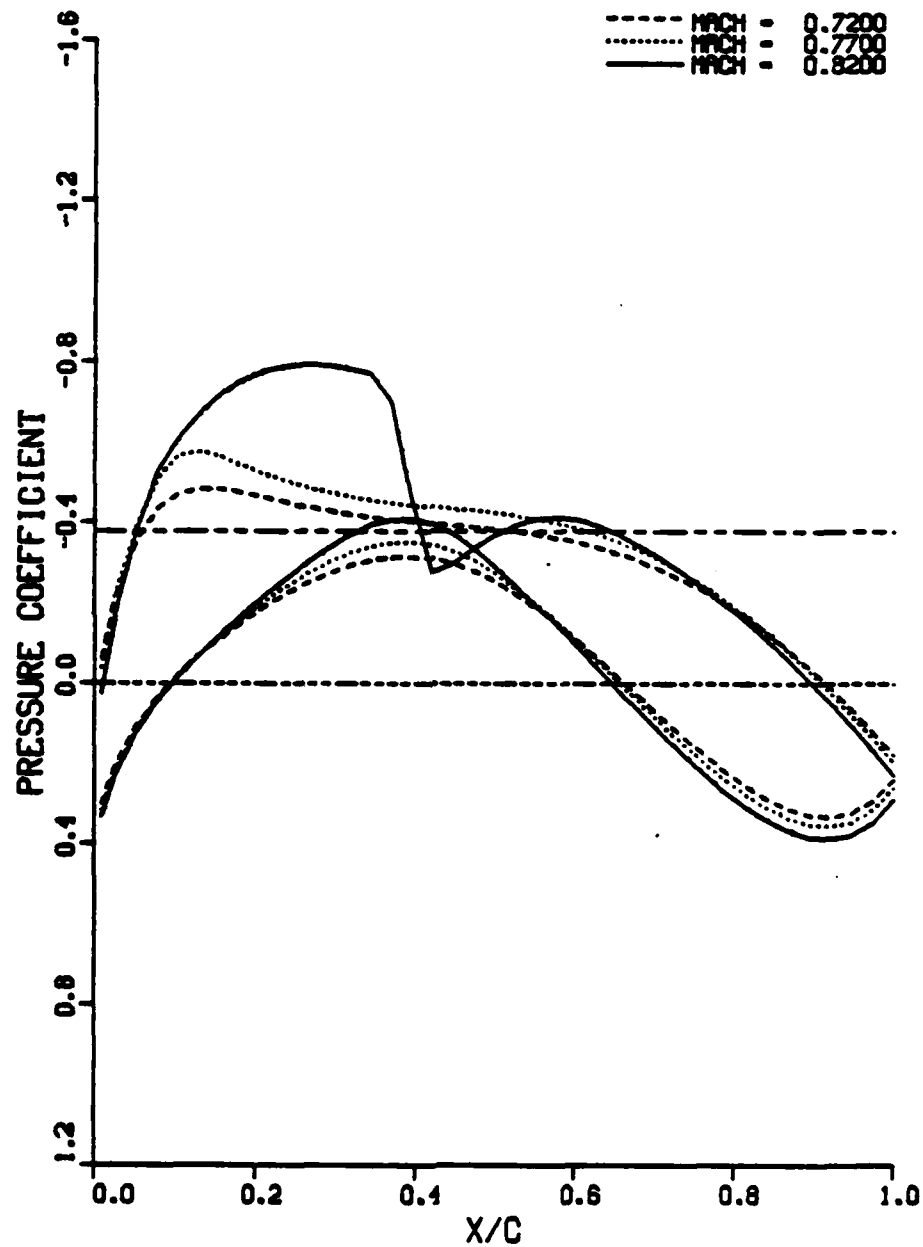
Figure 27. Effect of Mach Number Variation on Pressure Distributions for Fixed Mean Angle of Attack (Sheet 5 of 6)
