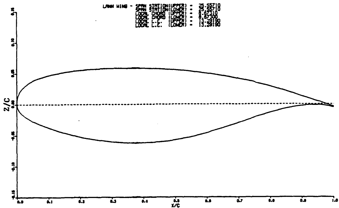
(e) SPAN-STATION = 0.65
