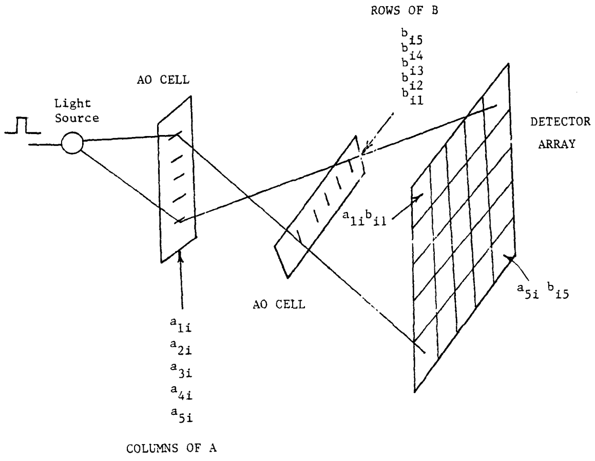
Fig. 3 - Outer product matrix-matrix multiplier using serial feed.
