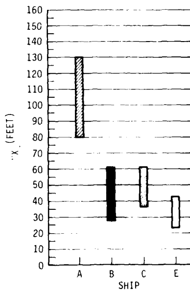
Figure 3-55. Confidence Interval of Population Mean (95%) 90° Turn - Consistency ( X_Q ) vs. Ship Type
