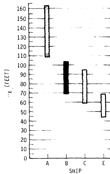
Figure 3-54. Confidence Interval of Population Mean (95%) Leg 4 - Consistency ( X_Q ) vs. Ship Type
