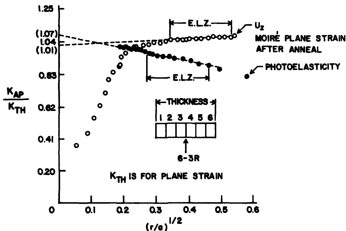
Fig. 4 Comparison of Photoelastic and Moiré Results.
