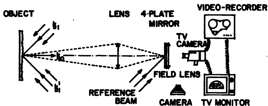
Fig. 10 Schematic representation of the recording system in image plane holography.
