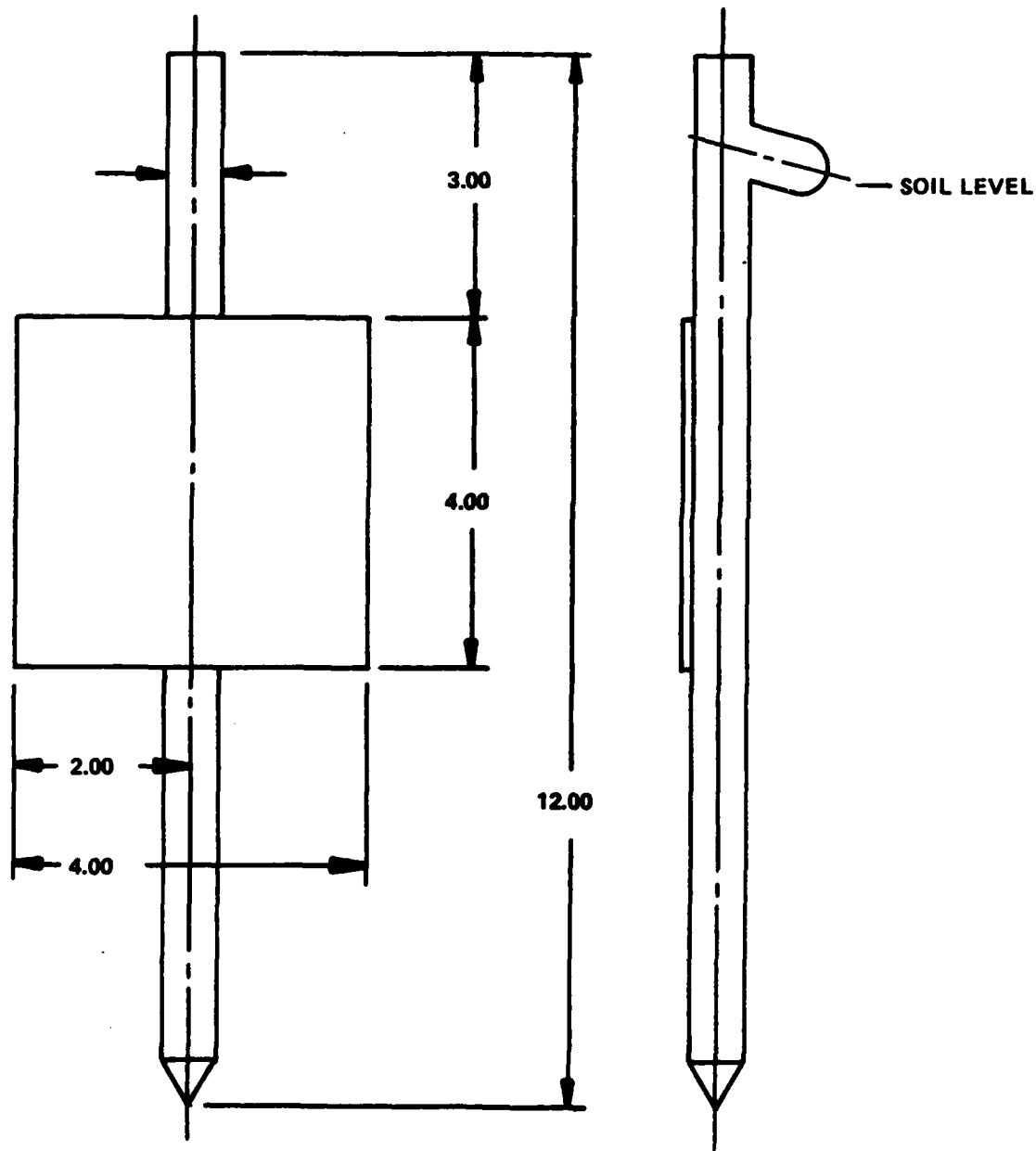
Figure 3 Stake Type 3
