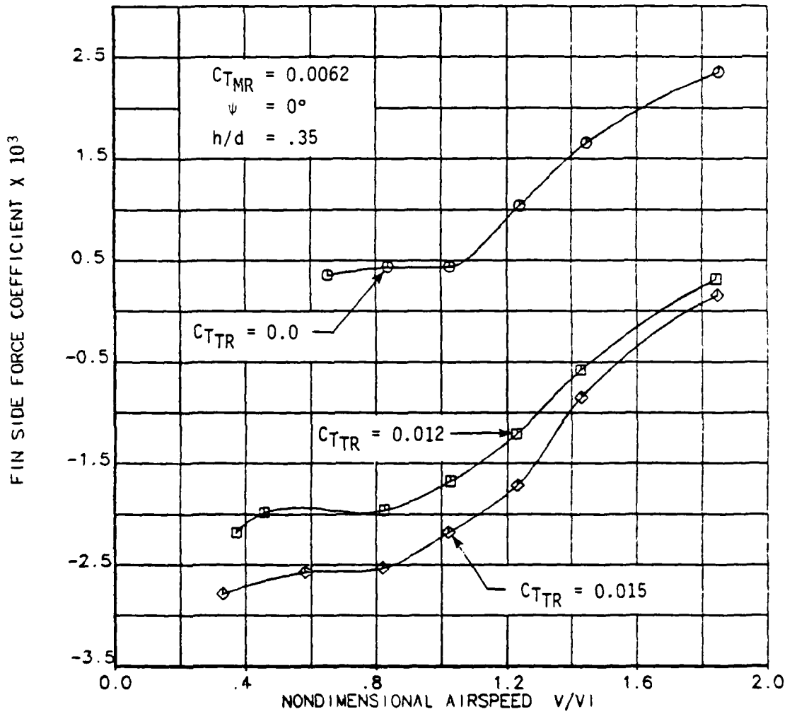
a. Forward Flight ( \psi=0 )
