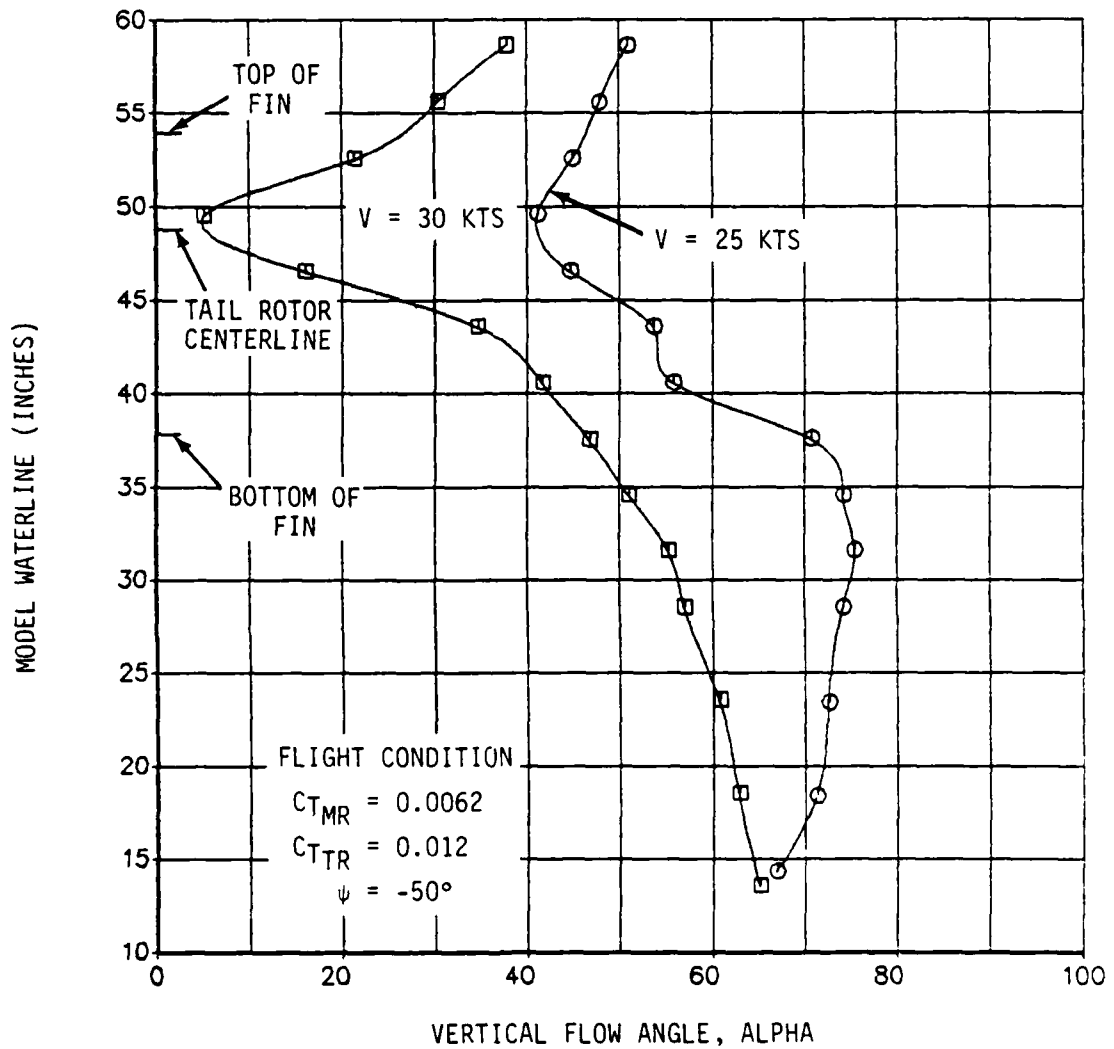
a. Vertical Flow Component
