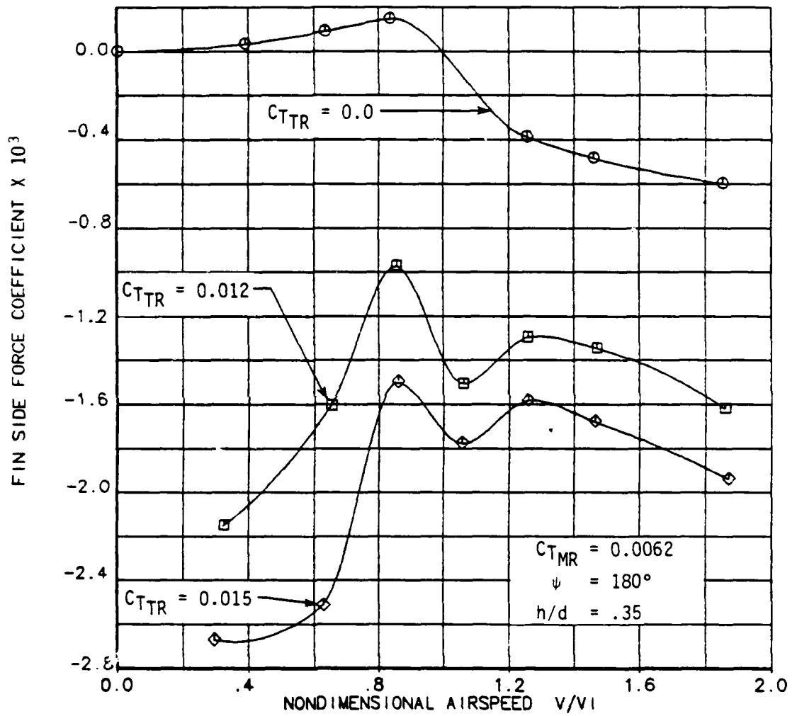
c. Rearward Flight ( \psi=180^\circ )
