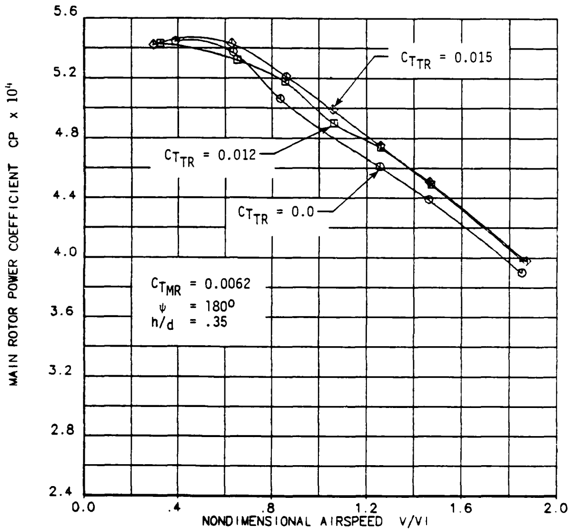
c. Rearward Flight ( \psi=180^\circ )
