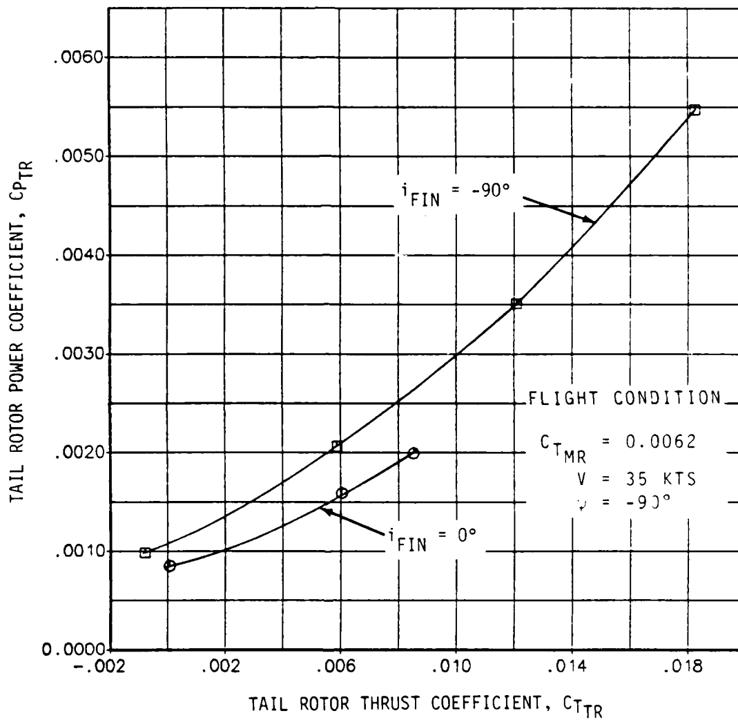
Figure 12. Effect of Varying Fin Incidence Angle on Tail Rotor Power in Right Sideward Flight
