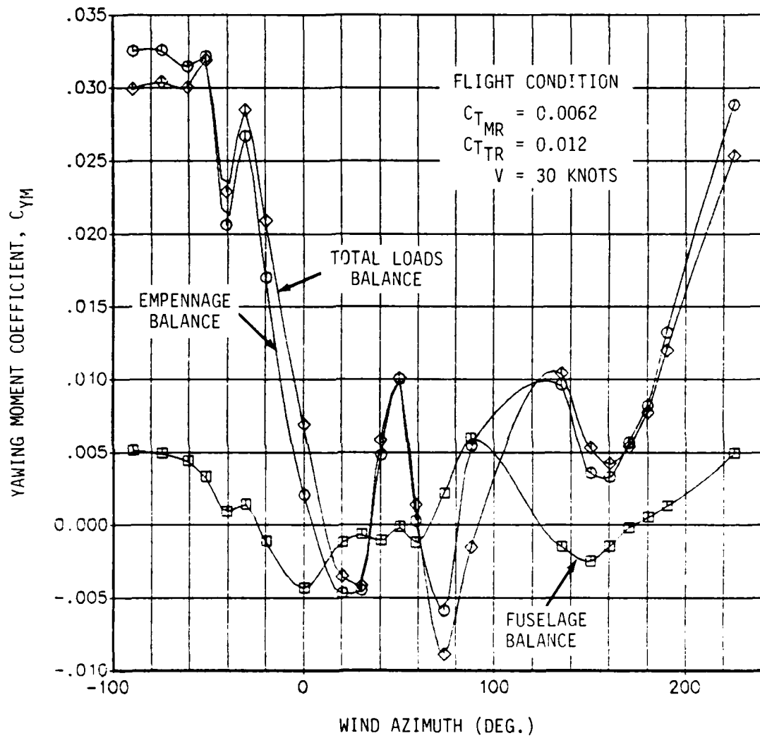
Figure 15. Component Breakdown of Yawing Moment Contributions as a Function of Wind Azimuth (referenced to model c.g.)
