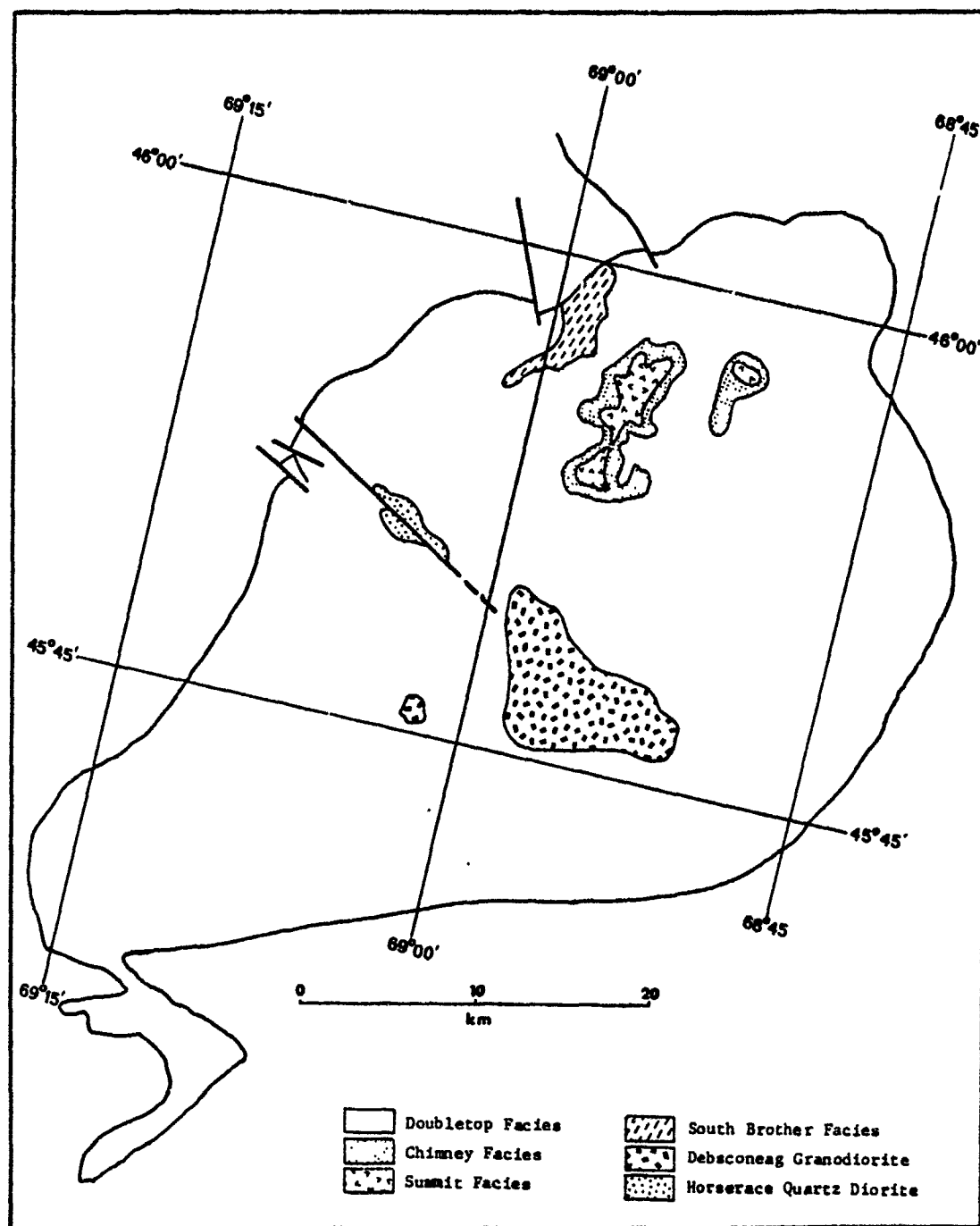
Figure 14. Geologic map of the Katahdin Pluton (After Hon, 1980).
