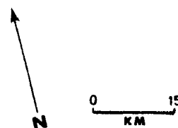
Plate 1. Study area, Kazakhstan, USSR. Image produced with principal components "2-2-2" method.
