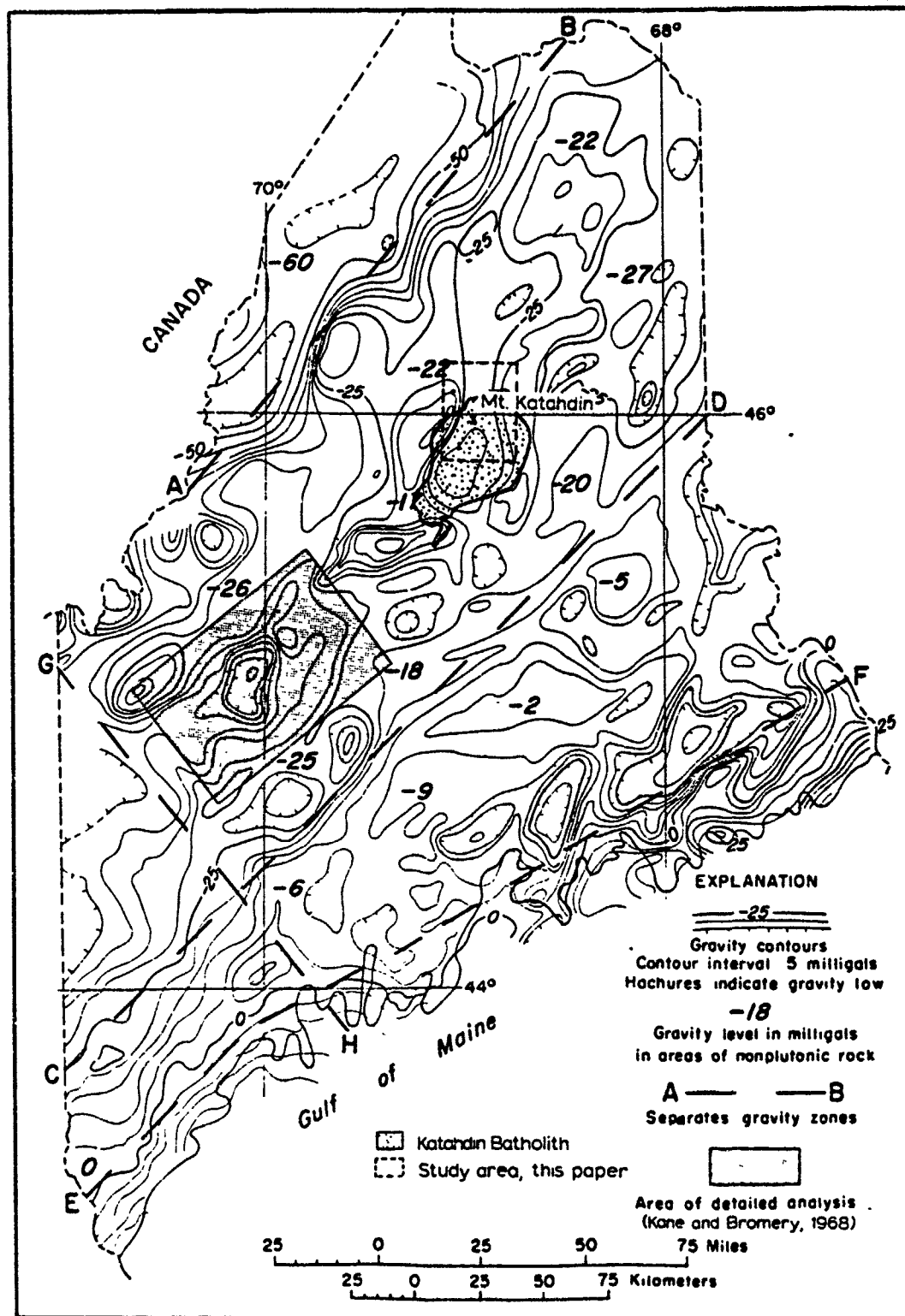
Figure 15. Bouguer gravity map of Maine (After Kane and Bromery, 1968).
