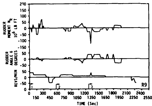
Figure 3-20 (c). Time Variation of Rudder Moment, Rudder Angle and RPM, Tug Forces and Moments, Active Tug Mode, Subject 7 (Cont), Runs R7 to R9
