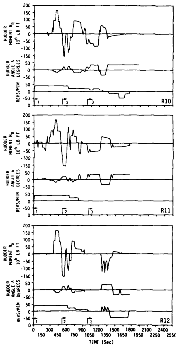
Figure 3-21 (d). Time Variation of Rudder Moment, Rudder Angle and RPM, Tug Forces and Moments, Active Tug Mode, Subject 8 (Cont), Runs R10 to R12
