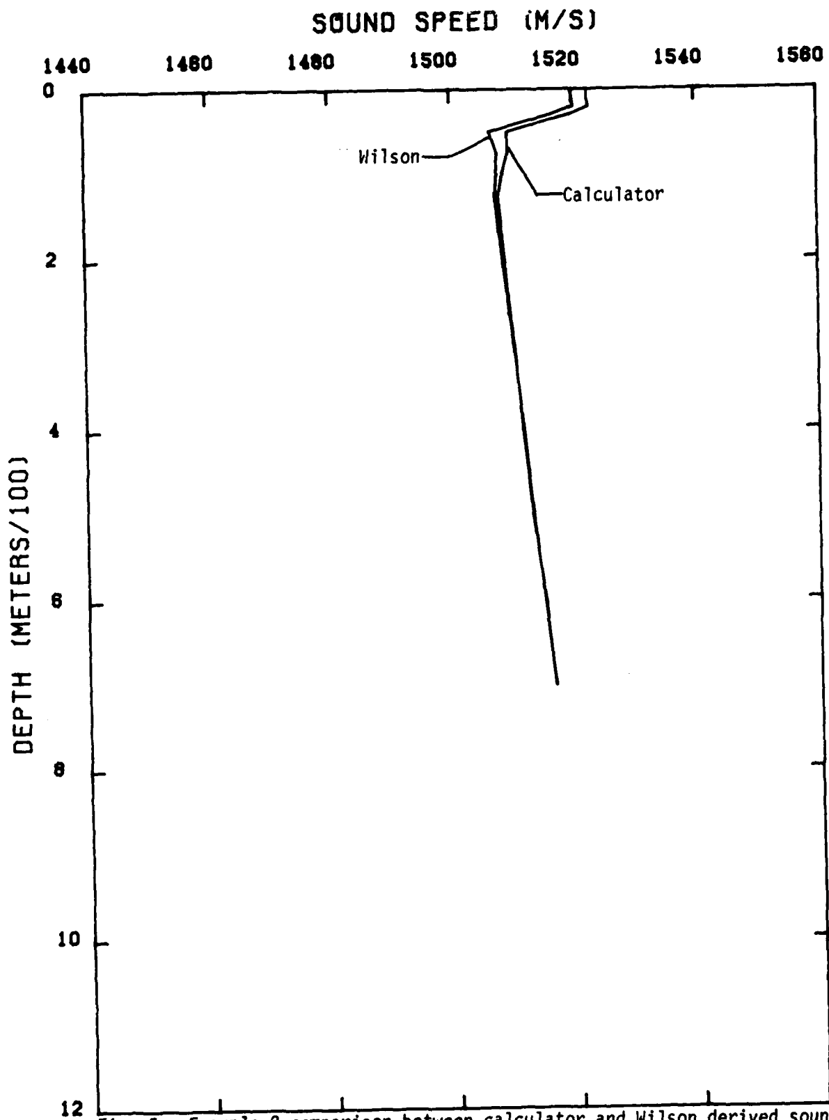
Fig. 5. Example 2 comparison between calculator and Wilson derived sound speed profiles.
