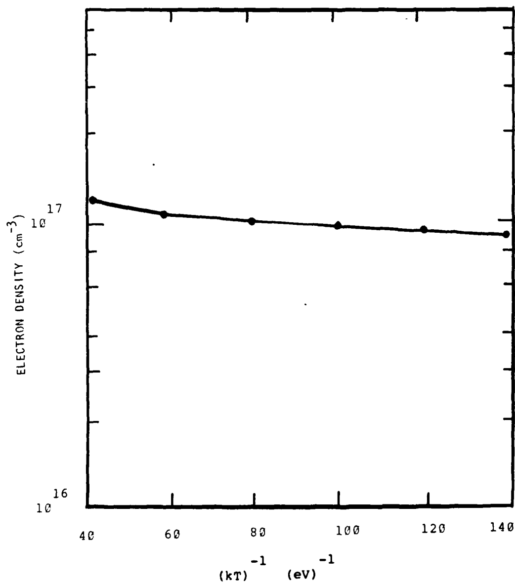
Fig. 3.11 Electron density vs inverse temperature for n-type InP.
