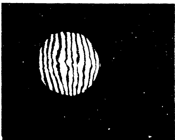
FRONT DISTORTION (SHEARING)
