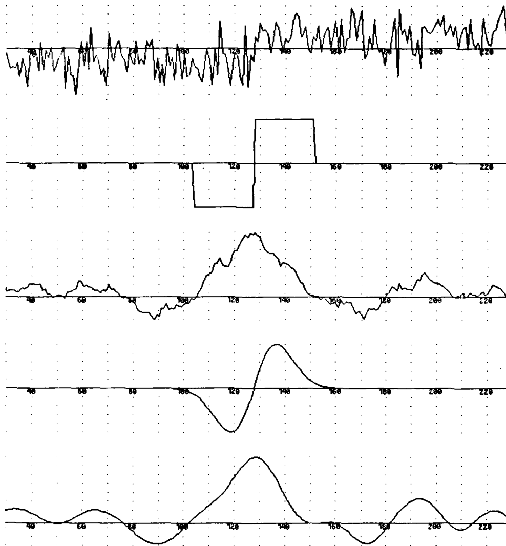
Figure 2.2. Responses of difference of boxes and first derivative of Gaussian operators to a noisy step edge
