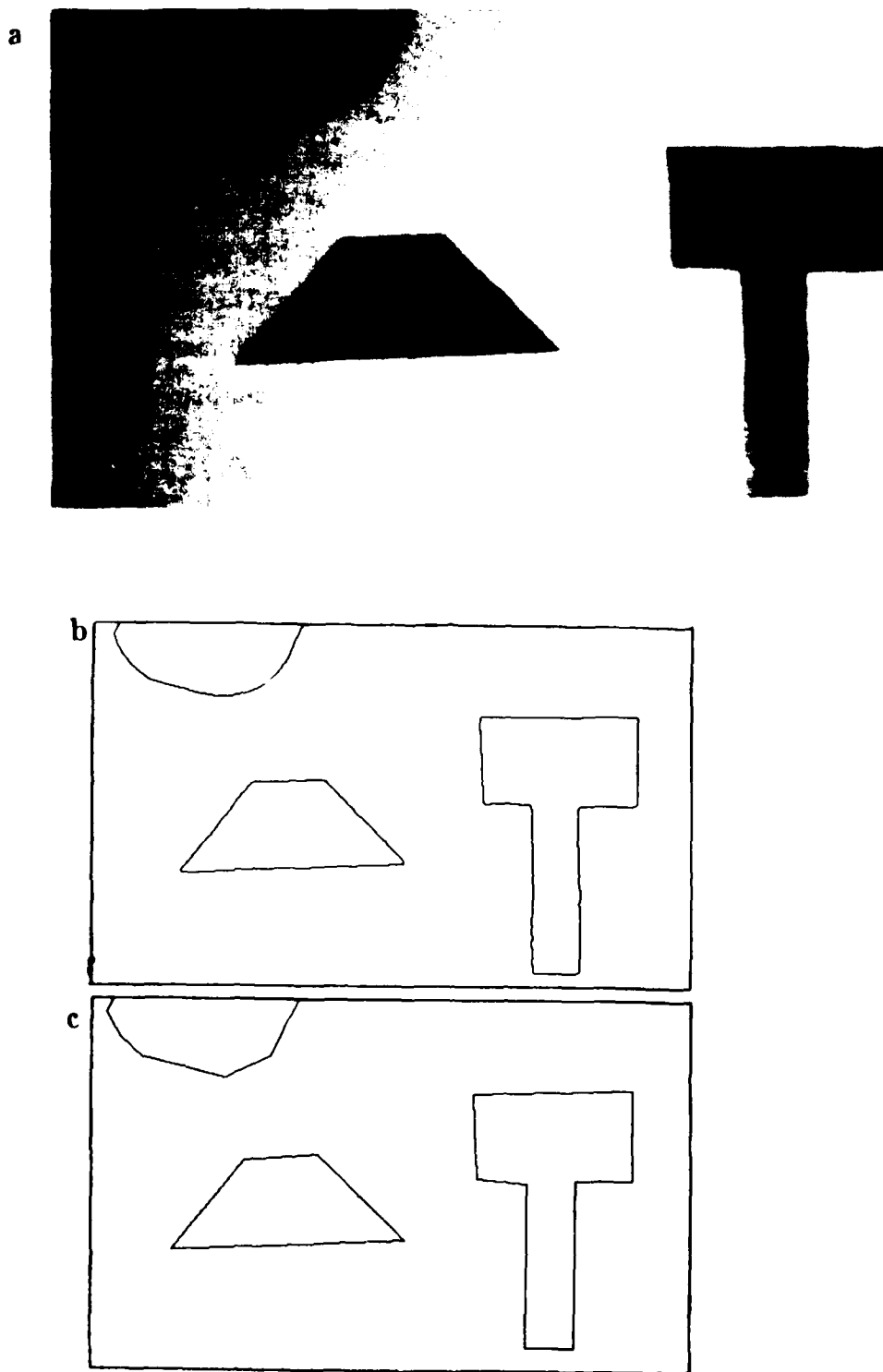
Figure 6.11. (a) Image of some paper shapes, (b) edges from operator width \sigma = 1.0 , (c) bounding polygonal approximation to the edges
