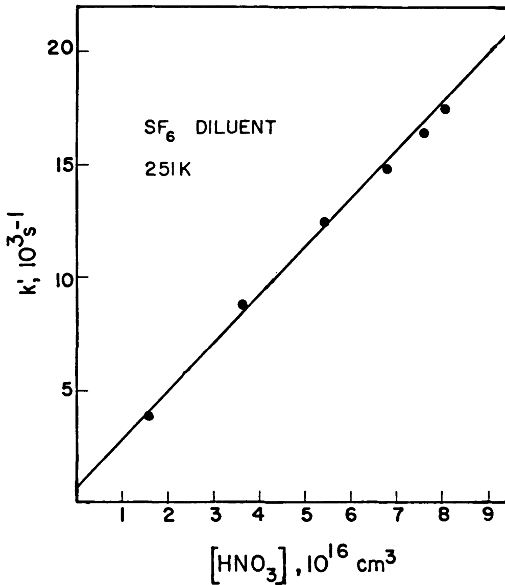
Figure 4. Plot of k' vs. HNO_3 Concentration Slope Gives the Rate Coefficient.
