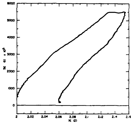
OIL PRESSURE VS DISPLACEMENT AT SOIL SURFACE (DYN/CM 2 VS CM)
