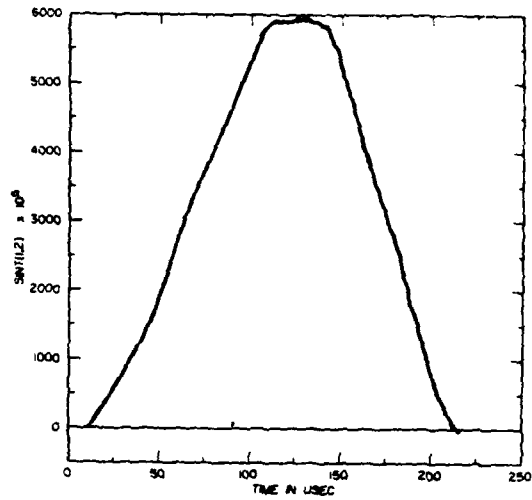
STRESS AT OIL-SOIL INTERFACE (DYN/CM 2 )
