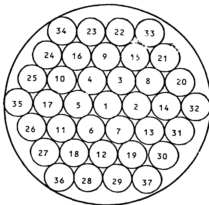
Figure 60. 37-wire multiwire bundle with labelling convention
