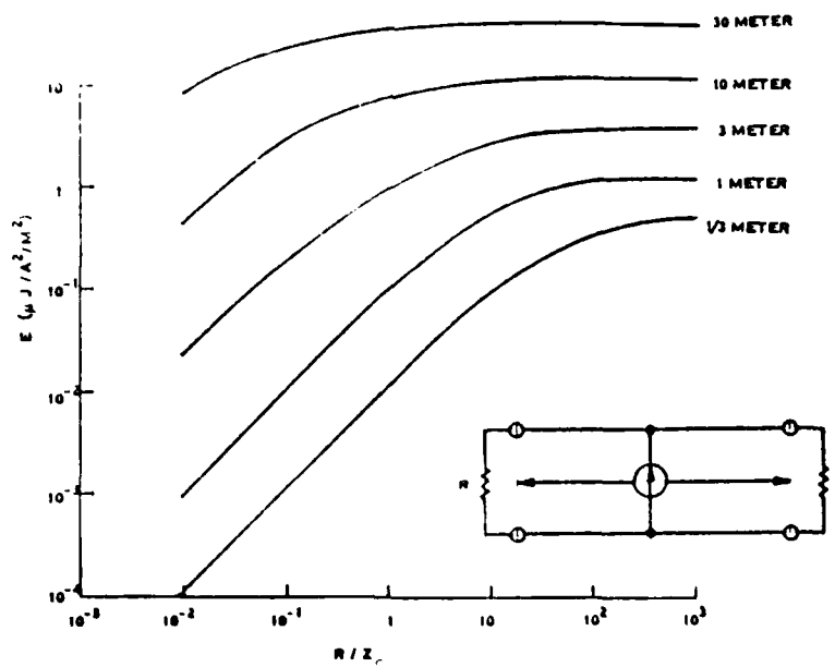
Figure 4. Transmission line dependence of the SGEMP energy delivered to component box interfaces from a 1 ampere per meter photon direct drive threat. The energy values shown are 50% of the final energy delivered.
