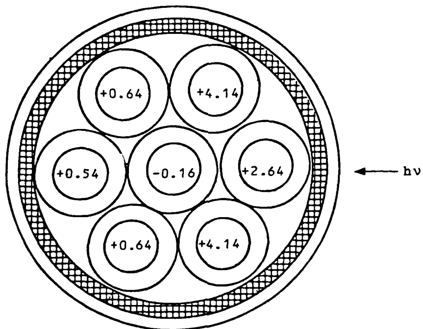
Figure 62. 7-wire current drivers
