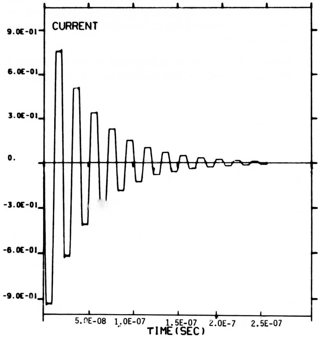
Figure 40. Terminal response - low mismatch
