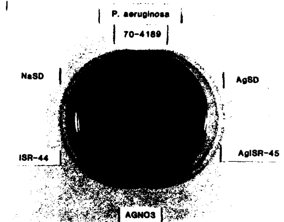
Fig 6.—Agar well assay of strain 70-4189. Silver nitrate (AgNO 3 ) is in center well. Wells contain test compounds at 50 mg/mL. For explanation of abbreviations, see legend for Fig 2.
