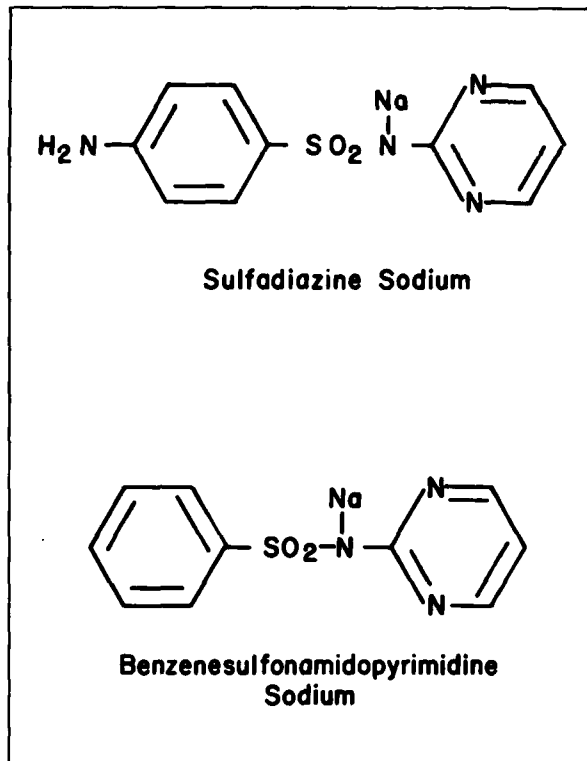
Fig 1.—Structures of sulfadiazine sodium and benzenesulfonamidopyrimidine sodium.
