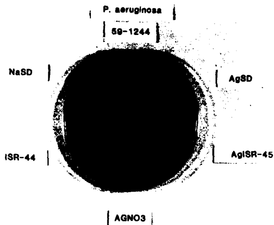
Fig 5.—Agar well assay of strain 59-1244. Silver nitrate (AgNO 3 ) is in center well. Wells contain test compounds at 50 mg/mL. For explanation of abbreviations, see legend for Fig 2.
