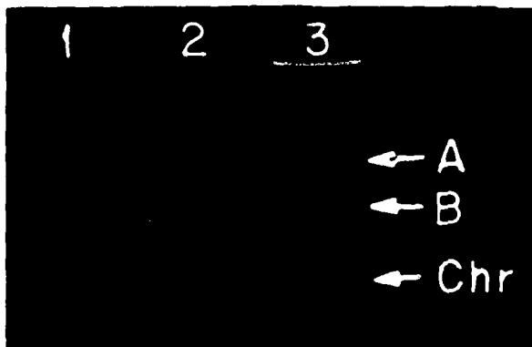
Fig 7.—Agarose gel electrophoresis of partially purified DNA from Escherichia coli C601 (track 1), Providencia stuartii (track 2), and transconjugate strain resulting after filter mating and selection for sulfonamide resistance transfer (track 3). Band A is plasmid DNA with molecular weight of approximately 80 megadaltons; band B, plasmid DNA with molecular weight of approximately 35 megadaltons; and band Chr, fragmented chromosomal DNA.
