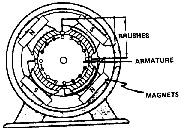
Figure 3-1 - D.C. Motor
