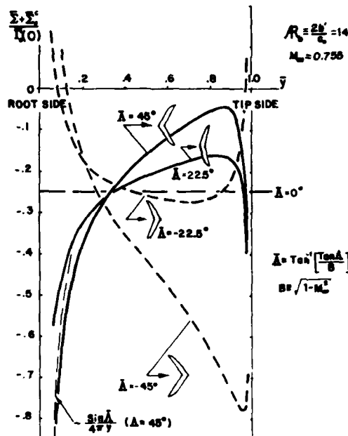
Fig. 3 Upwash function \bar{\Sigma} + \bar{\Sigma}_i illustrated for elliptically loaded swept-forward and swept-back wings of R_l = 14 at M_\infty = 0.755 . Refer to text for conversion to other aspect ratio and Mach numbers.
