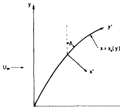
Fig. 1 Cartesian and orthogonal curvilinear coordinates in the wing plane z = z' = 0 .
