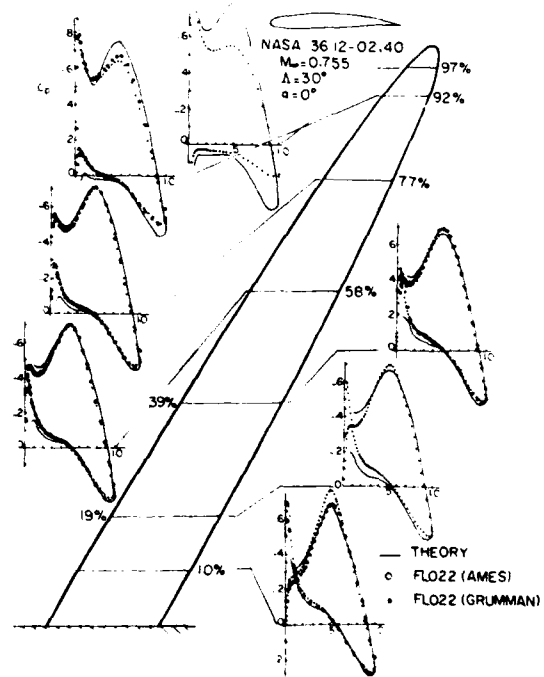
Fig. 6 Consolidated plot showing surface C_p on seven span stations of a symmetric swept-back wing with 30 deg sweep angle at flight Mach number of 0.755. The basic planform is a 14:1 ellipse; the wing section is NASA 3612-02, 40, zero incidence, zero twist, and no wing bend.
