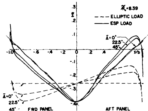
Fig. 2 Upwash function \Sigma illustrated for \sqrt{1 - M_\infty^2} R_l = 8.39 at three yaw angles for an elliptic and an extended span distribution in \Gamma_0 .
