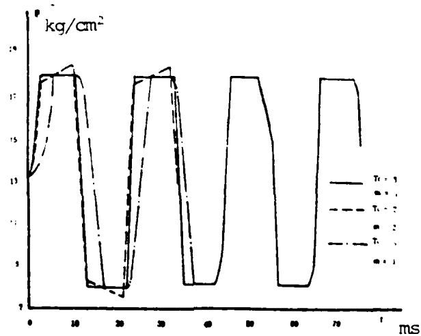
Figure 7. Curves of water impingement pressure in front of oxidizer valve after shut-down versus time.
