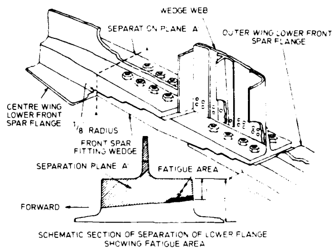
FIG. 7 MARTIN 2-0-2 WING ROOT FITTING FATIGUE FAILURE (Ref. )
