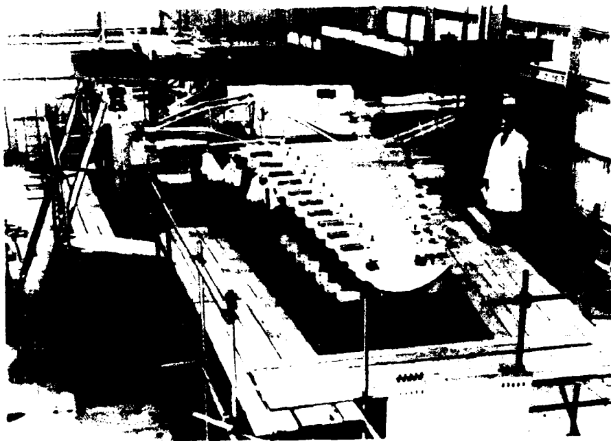
FIG. 4 "MOSQUITO" WING TEST RIG
