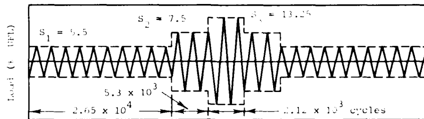
(a) Program block 3-load-level test (vibration rig)
