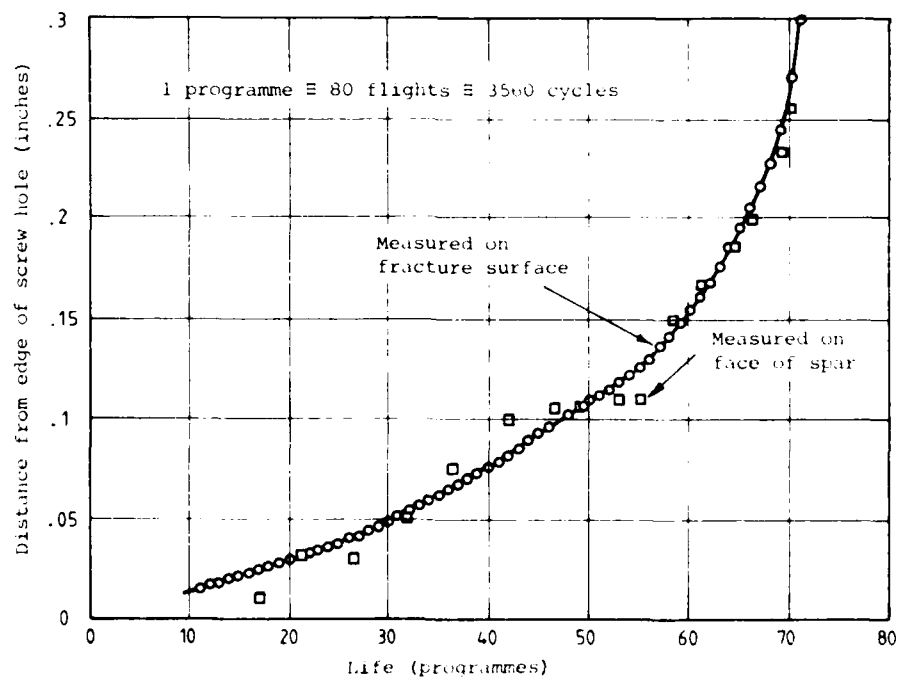
FIG. 13(b) CRACK LENGTH VERSUS LIFE, "VAMPIRE" SPAR (Ref. [1])
