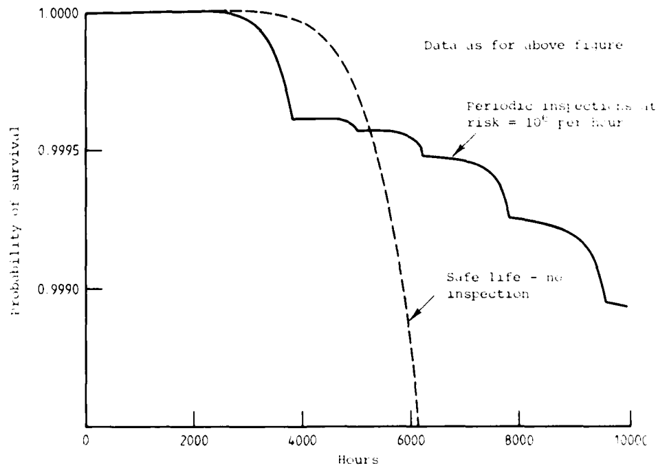
FIG. 18(b) PROBABILITY OF SURVIVAL vs LIFE (ref. 1)
