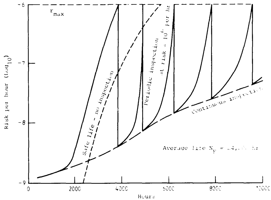
FIG. 18(a) RISK PER HOUR vs LIFE
