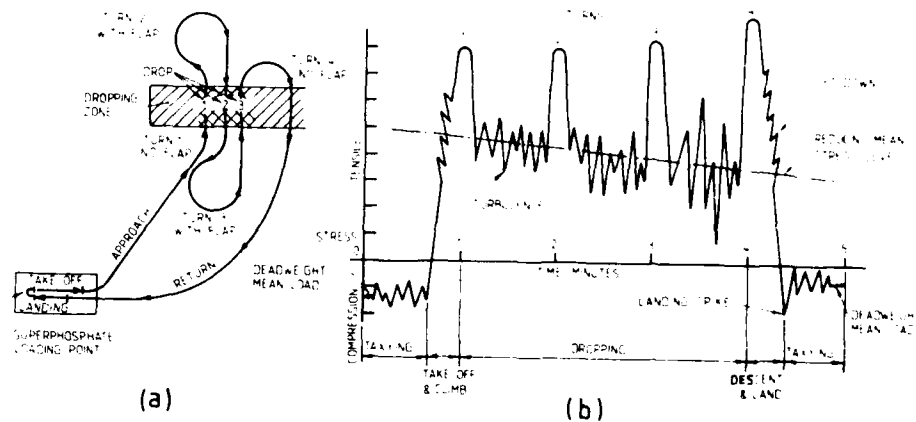
FIG. 15 (a) TYPICAL FLIGHT PATH FOR AERIAL AGRICULTURE OPERATIONS (b) STRESS-TIME PROFILE ON WING SPAR FLANGES FOR AIRCRAFT AT VARIOUS STAGES OF OPERATION (Ref. 1-1)
