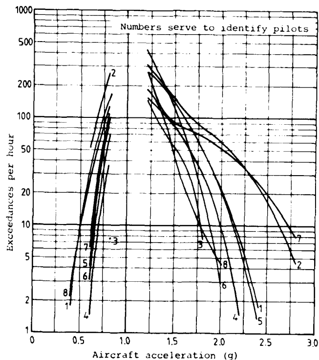
FIG. 16 VARIABILITY IN LOAD HISTORY CAUSED BY DIFFERENT PILOTS IN THE SAME AIRCRAFT (Ref. 1-10)
