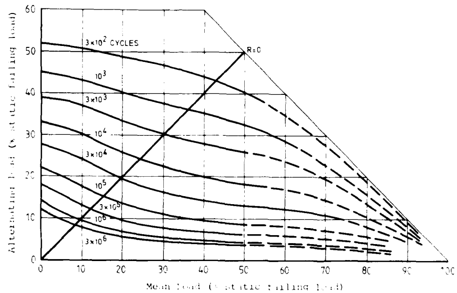
FIG. 9 ALTERNATING LOAD - MEAN LOAD DIAGRAM FOR MUSTANG WING FINAL FAILURE
