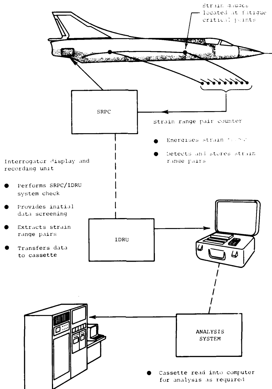
FIG. 17 THE AIRCRAFT FATIGUE DATA ANALYSIS SYSTEM (AFDAS)
