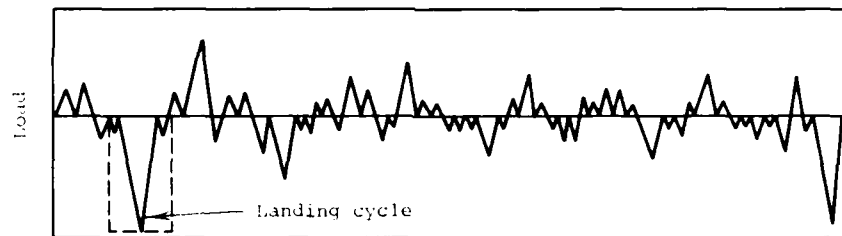
(c) Typical ground-air-ground cycle/gust load sequence (hydraulic rig)
