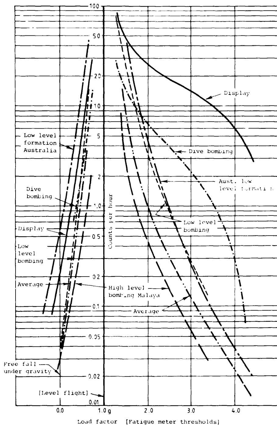
FIG. 12 LOAD-FREQUENCY CURVES FOR R.A.A.F. CANBERRA AIRCRAFT (Ref. 10)
