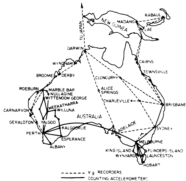
FIG. 10 FLIGHT LOADS MEASUREMENTS, AUSTRALIAN ROUTES-EARLY 1950's (Ref. 10)
