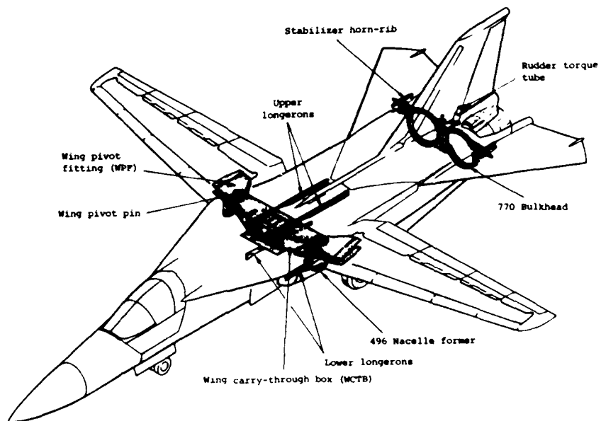
FIG. 19(a) D6AC STEEL STRUCTURAL MEMBERS IN F-111
