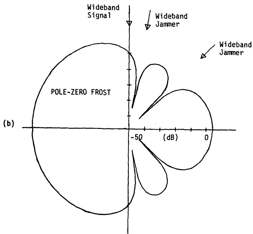
Fig. 17. Comparison of wideband antenna patterns for (a) conventional Frost and (b) pole-zero Frost. Both systems had essentially the same number of weights and convergence rates.
