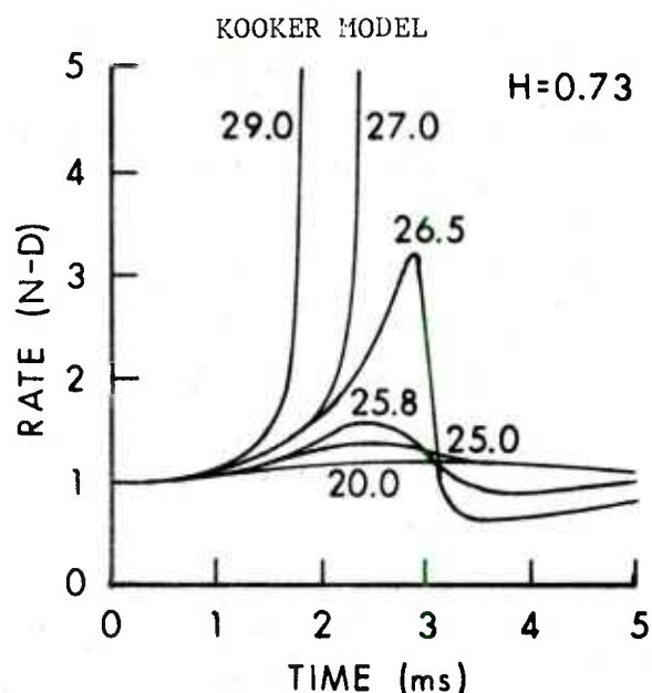
Figure 6. Effect of Activation Energy, Kooker Model
