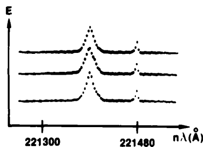
Fig. 2. Spectral distribution of three sequential laser pulses taken with the instrument described in Ref. 10. Each dot represents a channel of width n\lambda = 2.8 Å. To the right at n\lambda = 221480 Å is a He-Ne laser reference marker in 35th order. The pulsed laser is tuned to \lambda = 5534.8 Å and appears in 40th order at n\lambda = 221393 Å. For the pulsed laser each dot represents 0.07 Å. It is estimated that the center wavelength of the distribution varies about \frac{1}{2} of a channel.
