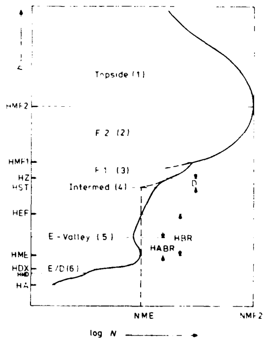
Figure 15d) N_e(h) model used in the International Reference Ionosphere.
