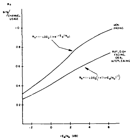
FIGURE 10 LOSS IN DETECTION EFFICIENCY DUE TO FADING
