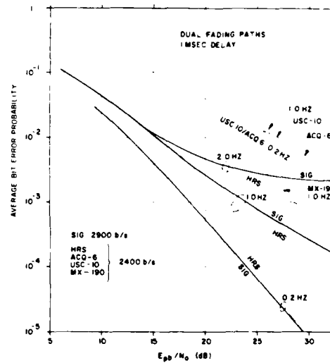
FIGURE 9 WATTEPSON TEST CHANNEL
