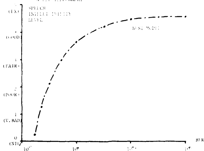
FIGURE 1.4: EMPIRICAL RELATIONSHIP BETWEEN LINCOMPLEX-PROCESSED SPEECH INTELLIGIBILITY & FSK TELEGRAPHY BER
