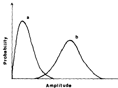
Figure 8 Schematic probability distribution of signal amplitude a) Rayleigh distribution from a random screen b) Rice distribution in the presence of a steady (specular) component (Davies 1969).
