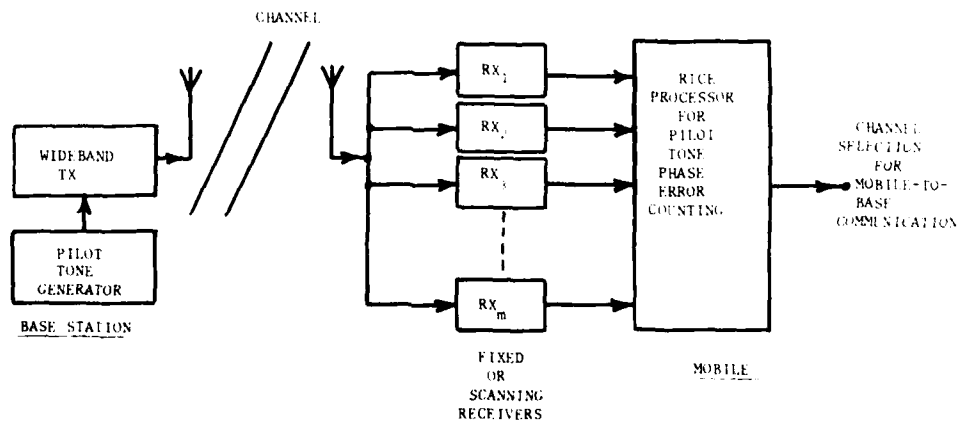
FIGURE 11: CLASS I APPLICATION OF PILOT TONE RICE
