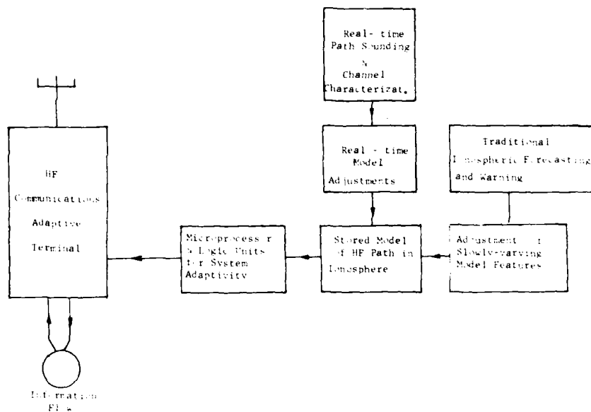
Fig. 1 Block diagram of an adaptivity approach that uses traditional HF ionospheric forecasting and warning, in addition to real-time path sounding and channel probing (taken from Aaron and Gross, 1982 [3])
