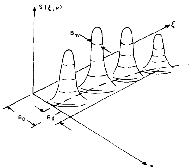
Fig. 3 Multimodal scattering function S(\xi, \nu)
