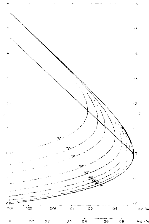
Figure 2 Normalized photoionization rate and electron density in a Chapman layer as a function of normalized height z and solar zenith angle \chi . z = \frac{h-h_0}{H} where h_0 is a reference height and H is the atmospheric scale height.
