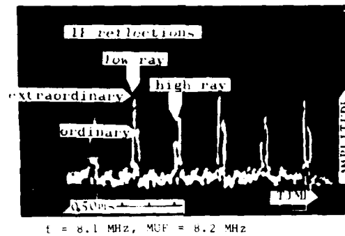
Figure 3 Multipath echoes from spread spectrum transmissions at 8.1 MHz (Lapp 1981).
