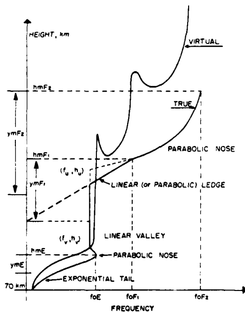
Figure 15c) N_e(h) model used in the IONCAP procedure
