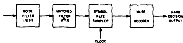
FIGURE 7 MLSE RECEIVER
