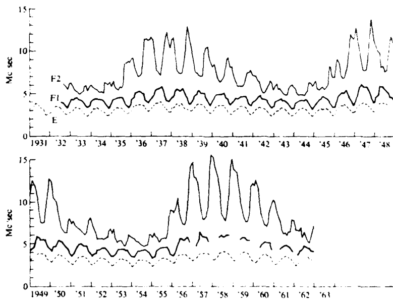
Figure 11 Long term variations of critical frequencies at Slough, England (Davies 1947).
