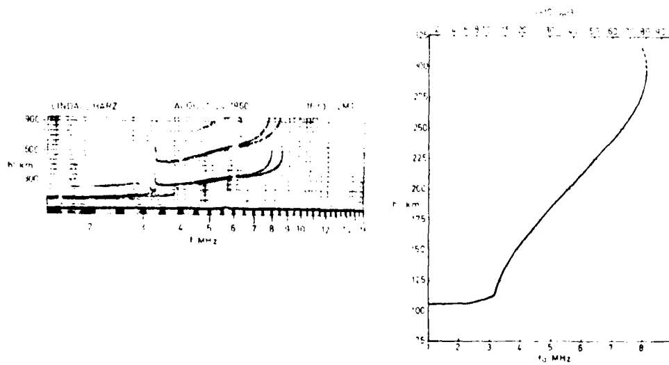
Figure 8 Typical ionosonde recording with corresponding electron density profile. (Lind et al 1967)
