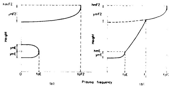
Figure 15a) N_e(h) model for CCIR first procedure. Figure 15b) N_e(h) model for CCIR second procedure.
