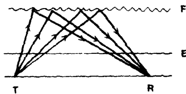
Figure 7 Illustrating reflection from an irregular ionosphere
