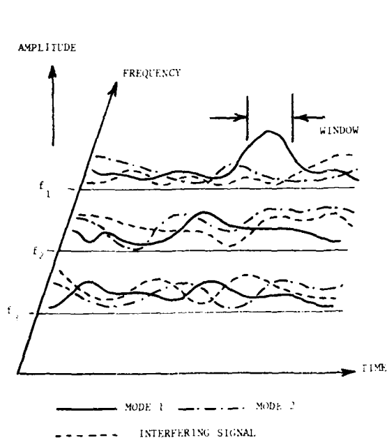
FIGURE 13: THE NATURE OF A VARIABLE CAPACITY HF PATH
