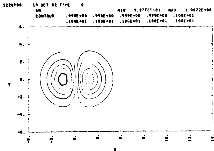
Figure 3-4. The neutral density after 10 seconds of initial evolution.
