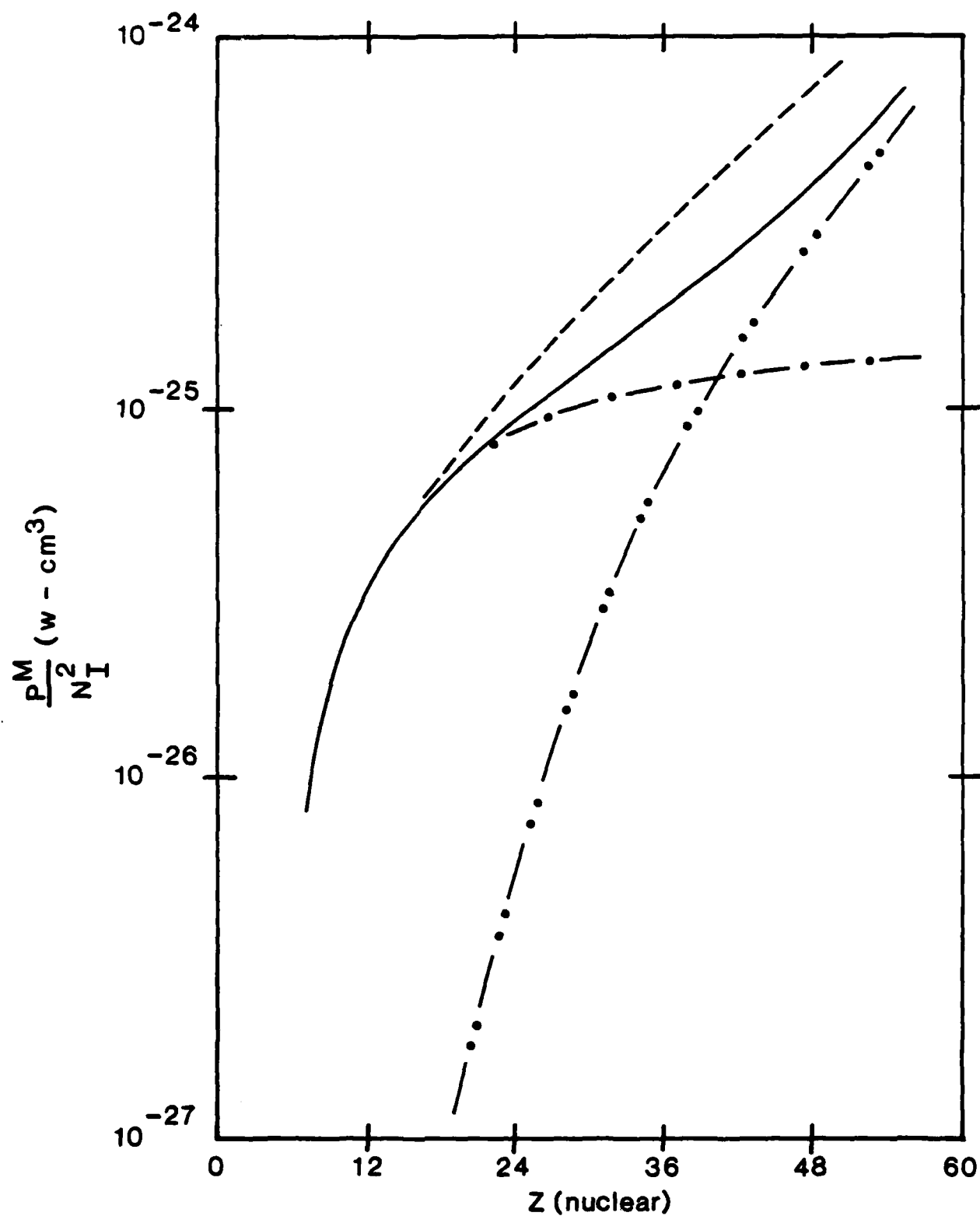
Figure 4. Radiated Power
