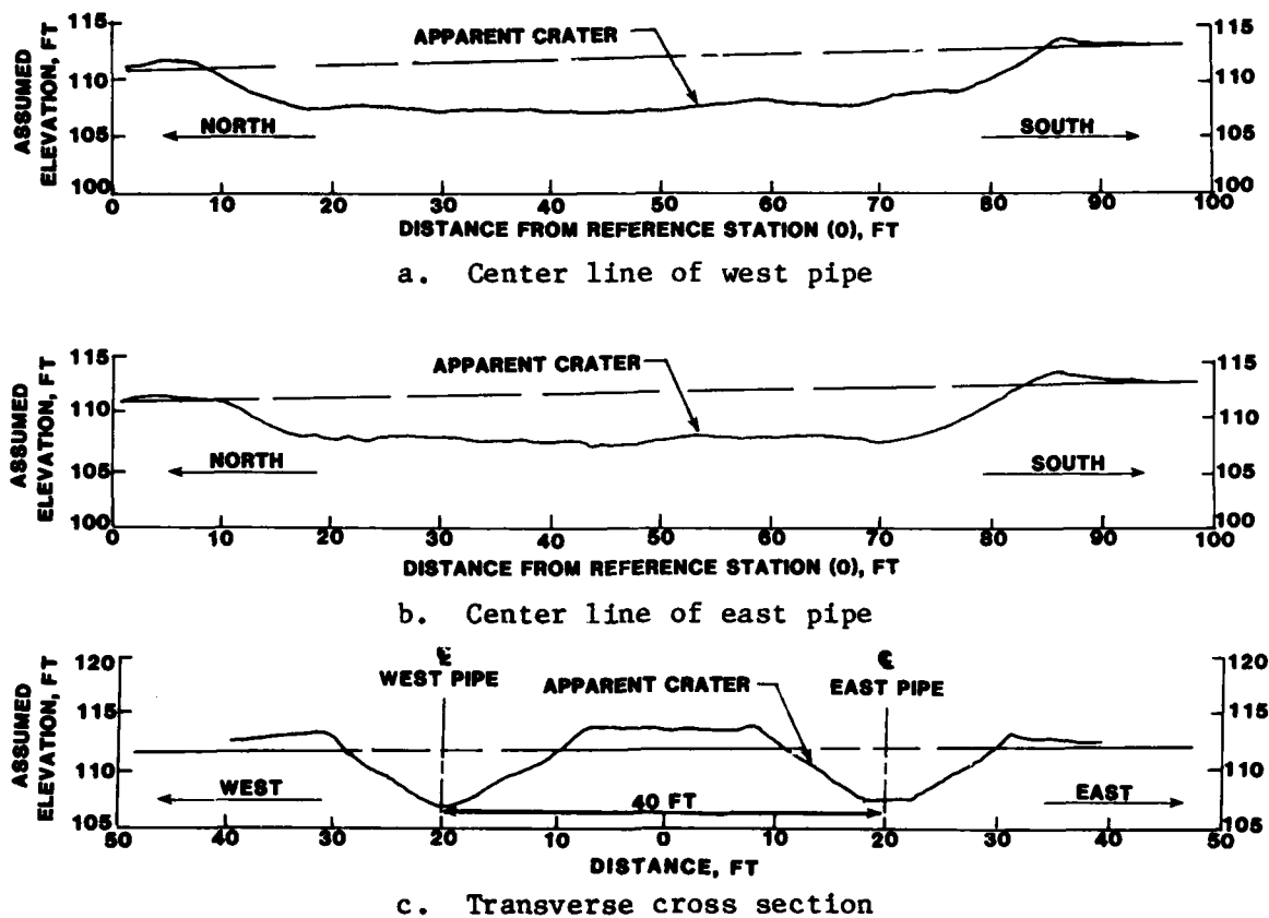
Figure 28. Double ditch shot 6SDR1, showing center-line and transverse profiles. Transverse profile is at midlength of ditch
