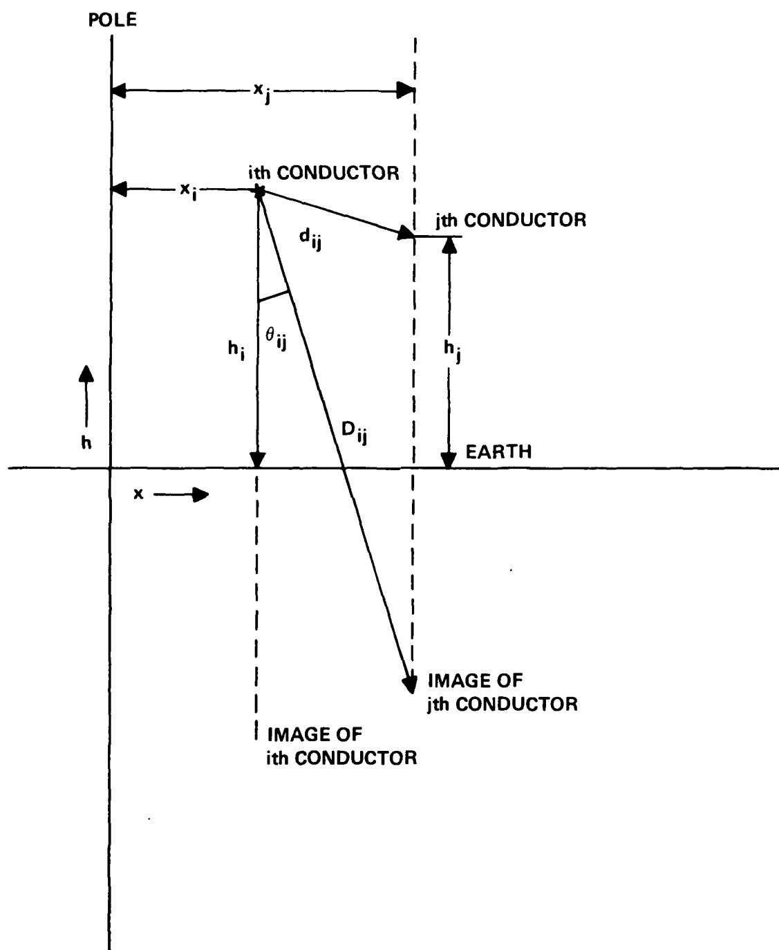
Figure C-1. Conductor-earth geometry.
