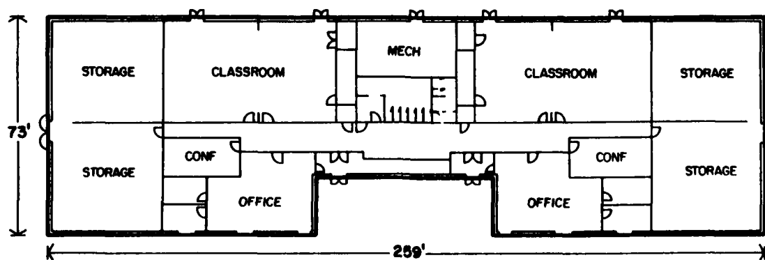
Figure 9. Battalion headquarters and classroom building floor plan.
