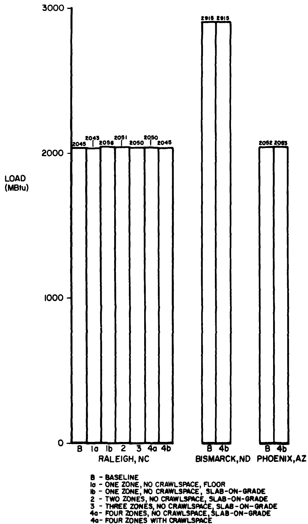
Figure 19. Total loads, dental clinic.
