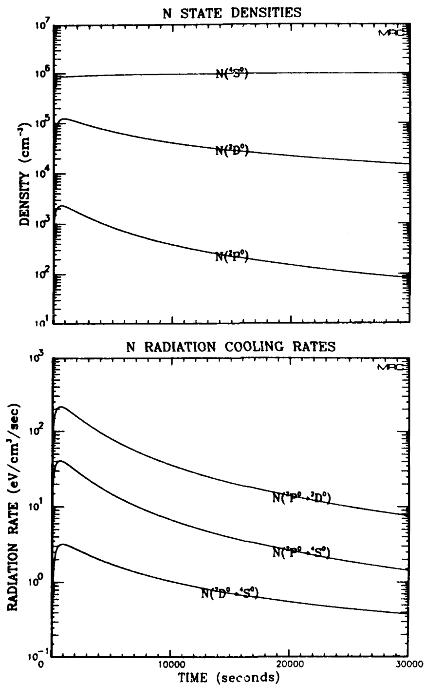
Figure 14. Radiation properties of N atoms at an electron density of 10^6 \text{ cm}^{-3} .
