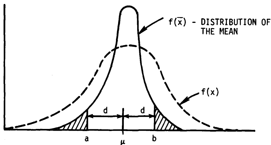
FIGURE 9: THE DISTRIBUTION OF THE MEAN OF A NORMAL
