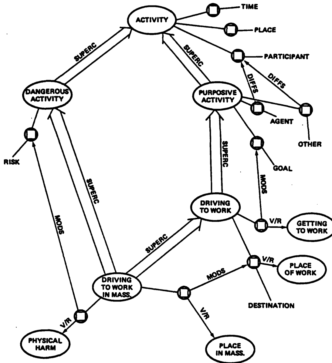
FIG. 1. AN EXAMPLE OF A KL-ONE NETWORK.
