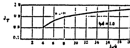
Fig. 11 Taylor correction factor from 2 to 3 dimensional motion.
