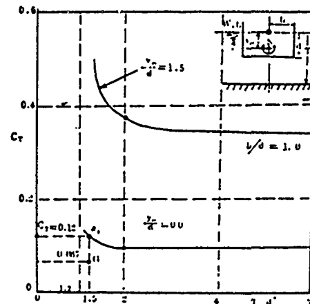
Fig. 9 Effect of shallow water on added mass moment of inertia in rolling (after Matsuura & Kawakami).
