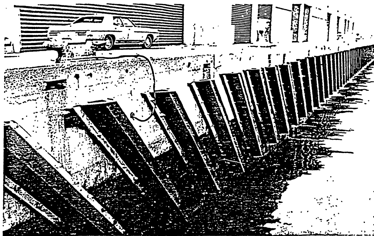
13" high Wing Type Trapezoidal fenders, 10 ft. long mounted diagonally on pier. Northeast Terminal, New York, N.Y.
