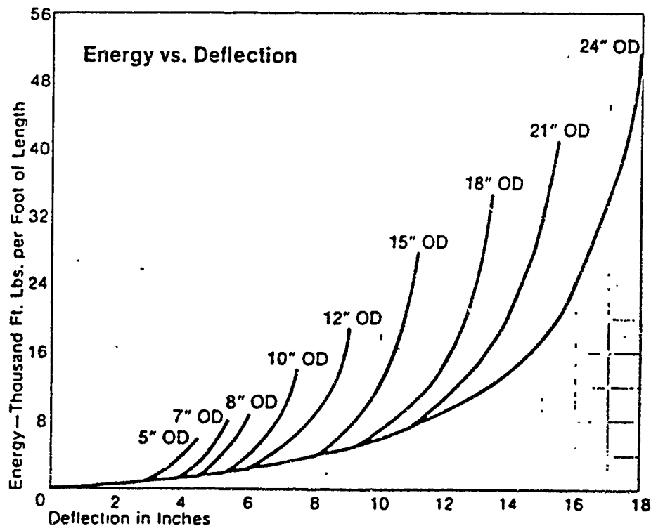
Approximate energy vs. deflection
