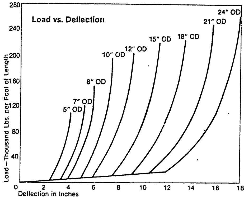
Approximate load vs. deflection
