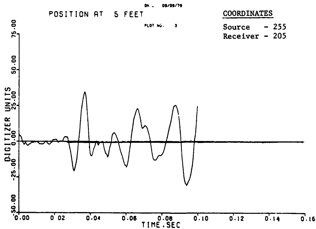
Figure 20. Digitized oscillograms for constant-spacing tests along 80W line, positions 0 and 5 ft
