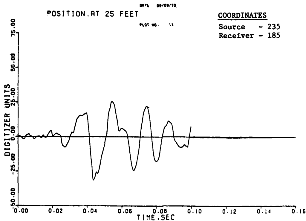
Figure 22. Digitized oscillograms for constant-spacing tests along 80W line, positions 20 and 25 ft
