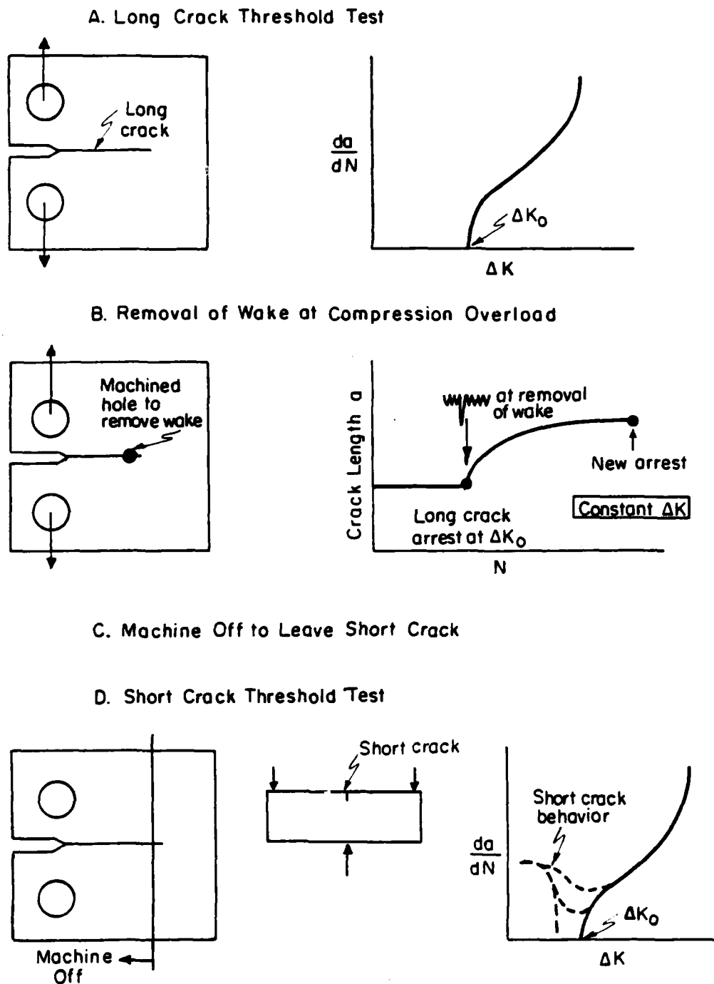
Fig. 3: Test geometries, procedures, and expected results for the "3 in 1" specimen developed to experimentally demonstrate the role of closure and the differences between long and short crack behavior.
