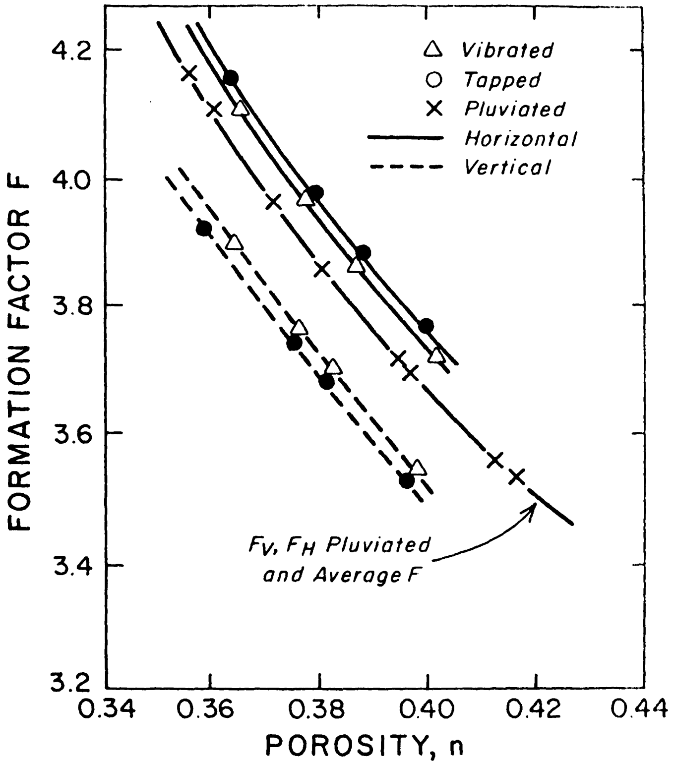
Fig 1. Formation Factor and Porosity Relationship for Lucite Balls
