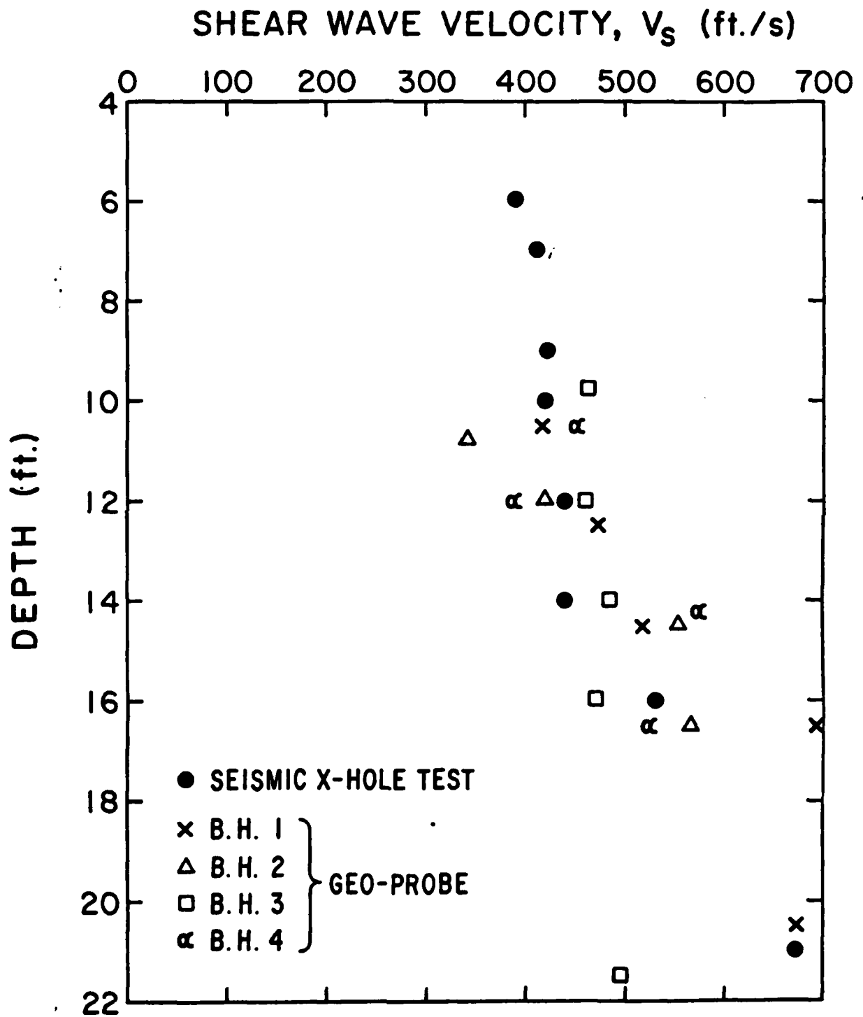
Fig. II. COMPARISON OF SHEAR WAVE VELOCITIES OBTAINED FROM CROSS-HOLE MEASUREMENTS AND USING GEO-PROBE FOR EL CENTRO SITE
