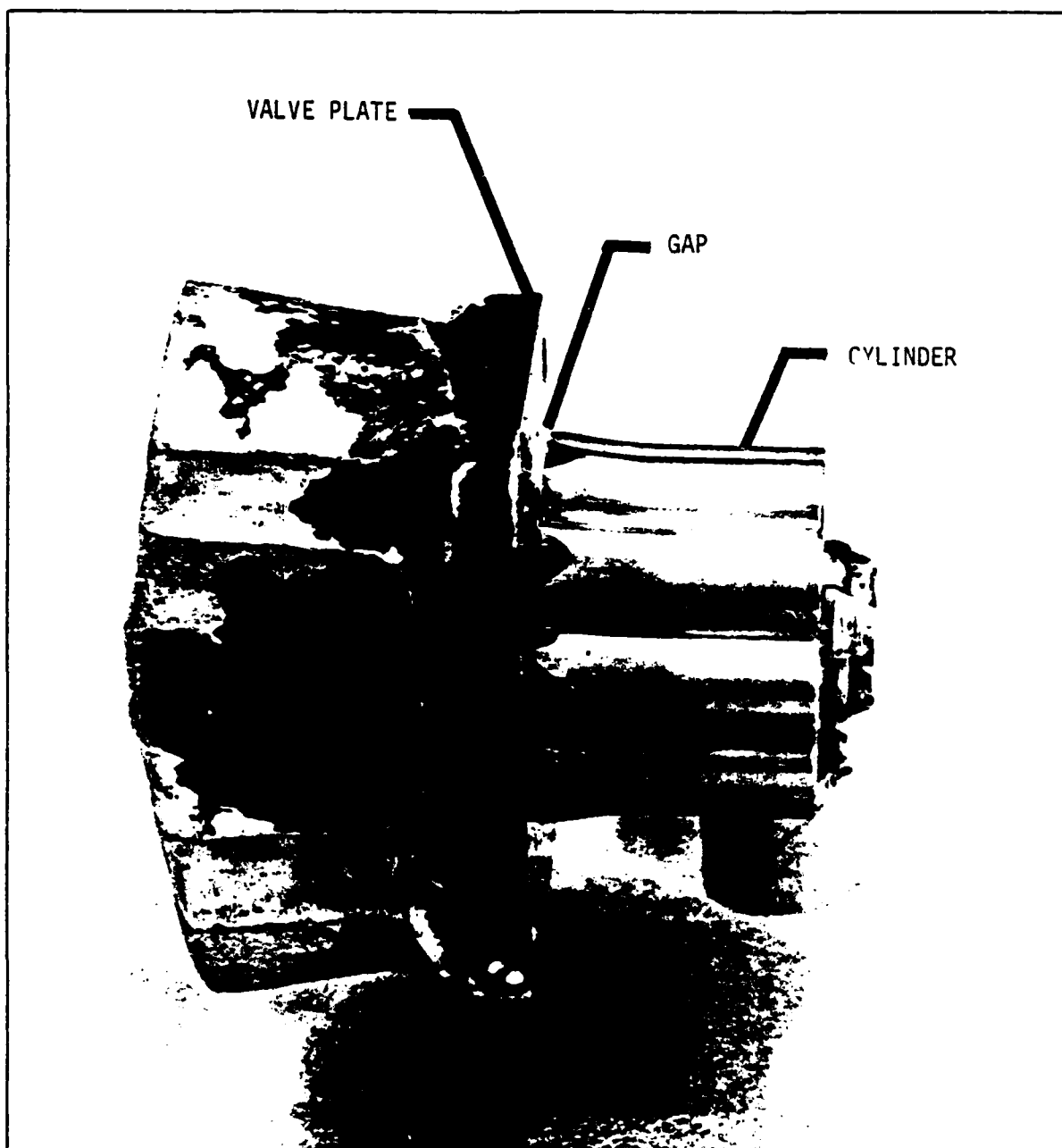
Figure 6 - Failed Motor Valve Plate and Cylinder Gap
