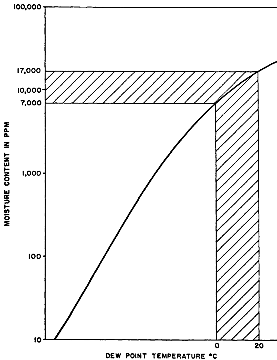
FIGURE 10. DEW POINT RANGE FOR FAILED RESISTORS
