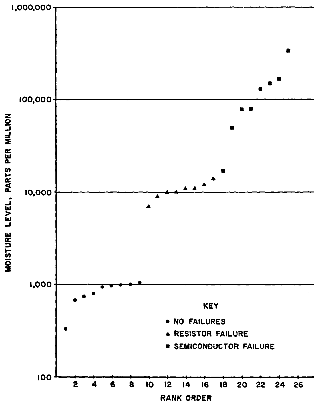
FIGURE 9. FAILURE MECHANISM VS MOISTURE CONTENT
