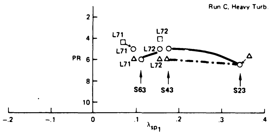
Figure 13 (3.2.1.3). Pilot Rating vs Unstable Root ( \lambda_{sp1} ) for \lambda_{sp2} = -2.0
