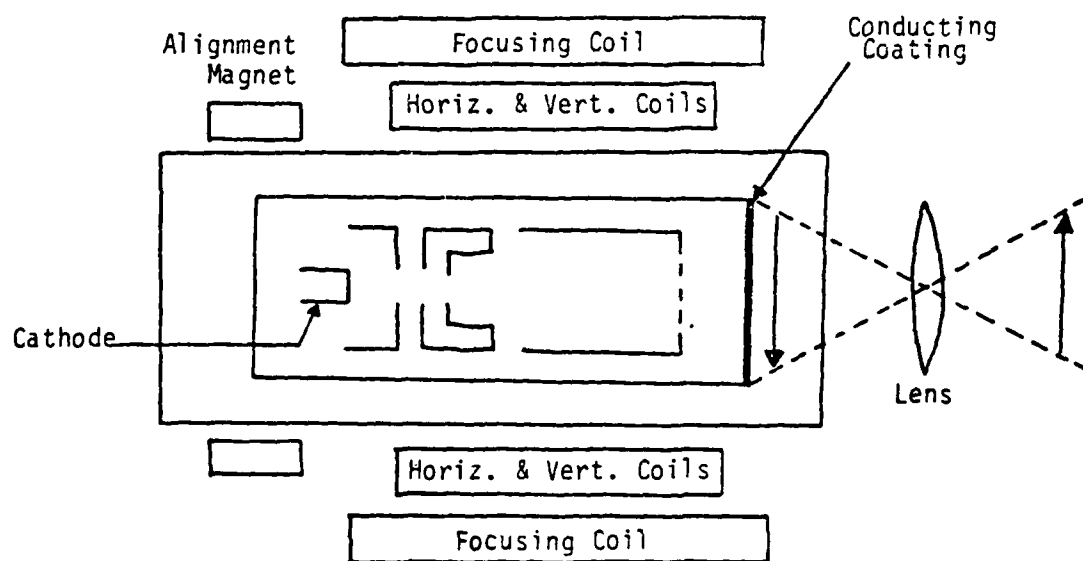
Figure 2.3 A Vidicon Tube.
