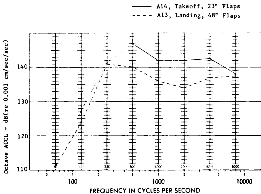
FIGURE 27 FUSELAGE WALL VIBRATION DURING TAKEOFF AND LANDING
