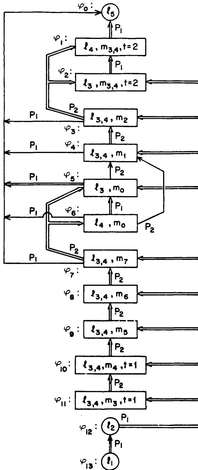
Fig. 1. Proof Diagram for the Mutual Exclusion Program
