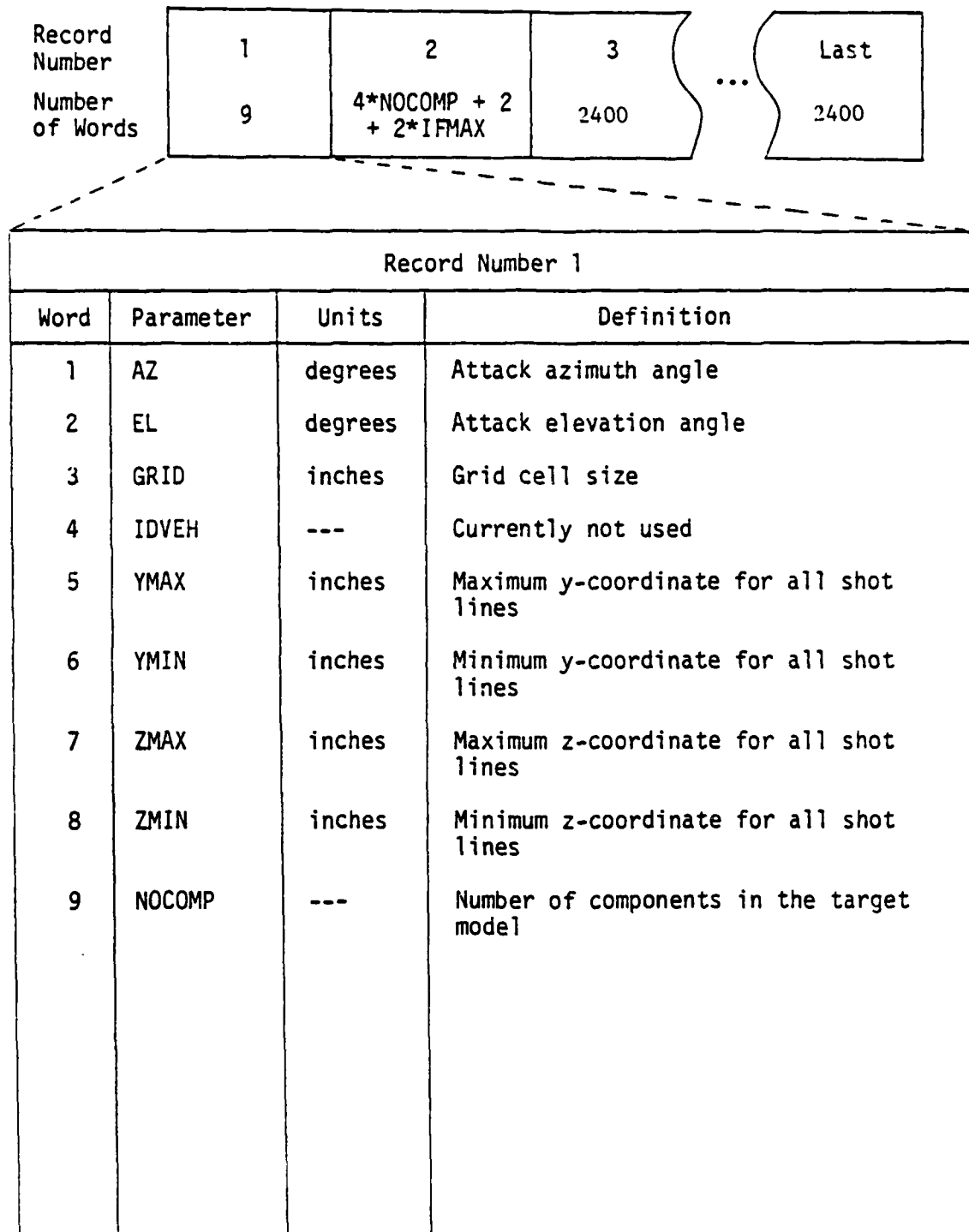
FIGURE 5-3. PEAKAY Binary Input, Viewing Plane Description.
