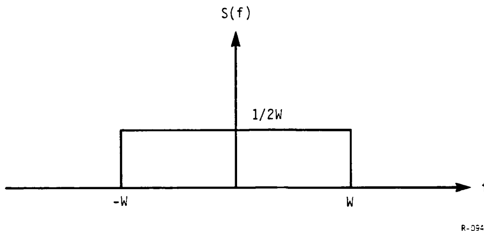
Figure 3-1. Signal Spectrum.
