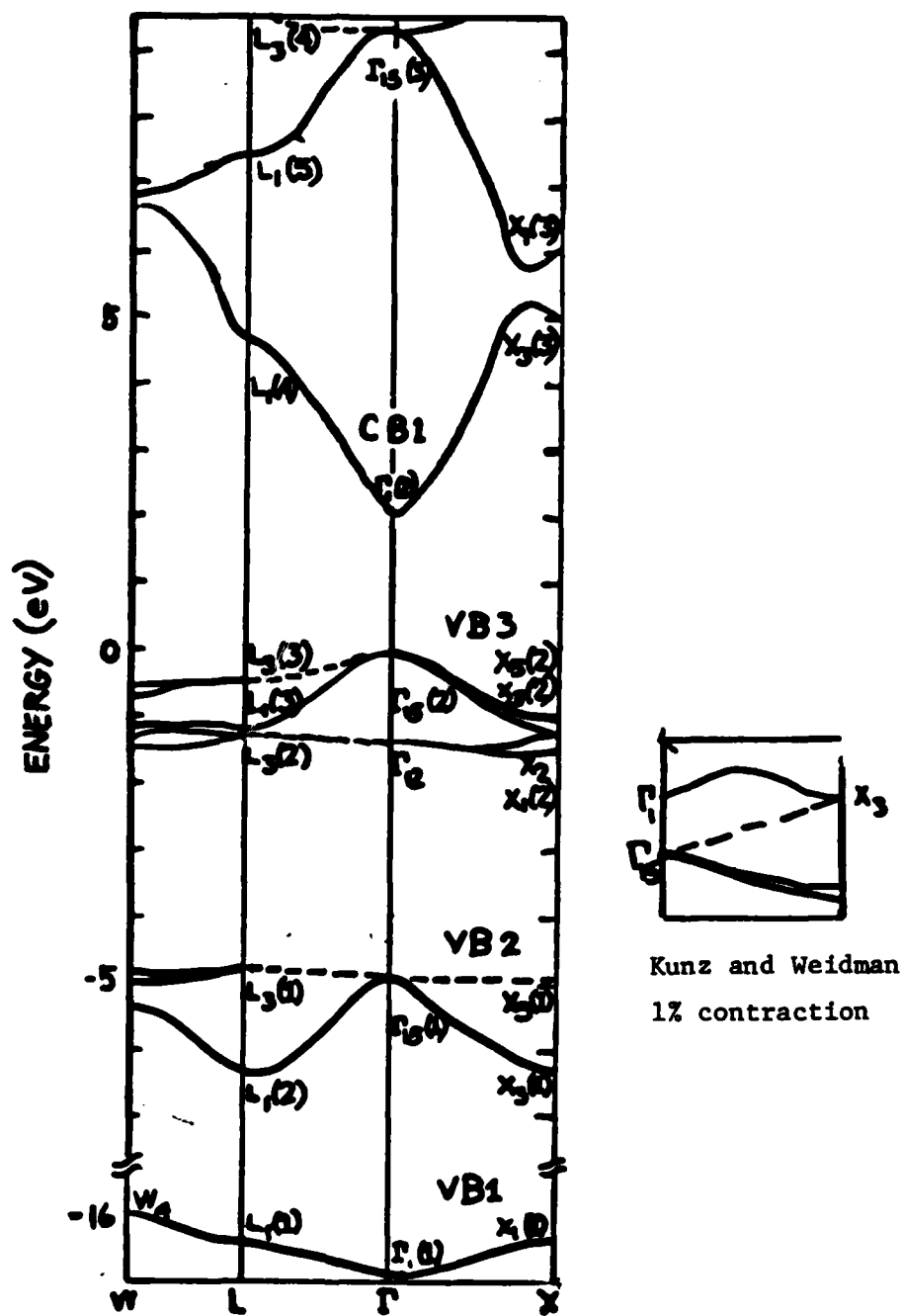
Figure 1. Equilibrium energy bands of CuCl.
