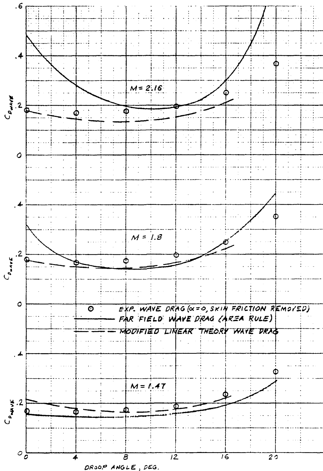
Figure 19 - Drooped Nose Body Drags
