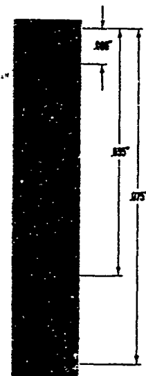
Figure 3b. Transverse Cut Through an Engraved Groove of a Rotating Band of a 105 mm Projectile - Reduced 50 Percent from 100X Magnification.
