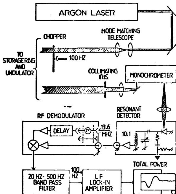
Figure 2 : Simplified schematic diagram of experiment.
