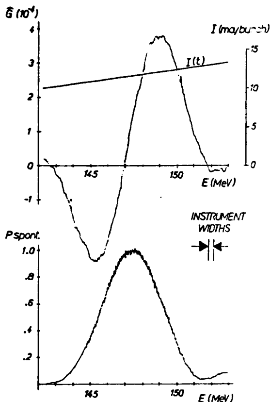
Figure 3 : Gain and spontaneous spectrum vs energy.
