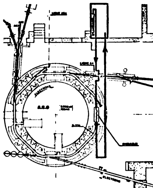
Figure 1 : Placement of undulator and gain measurement beam lines.
