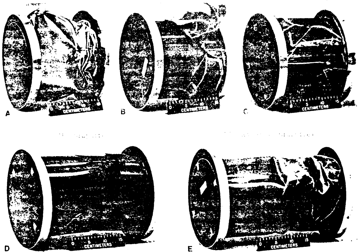
Figure 3.6. Internally-Strained Specimen After Failure (See Fig. 3.5)
