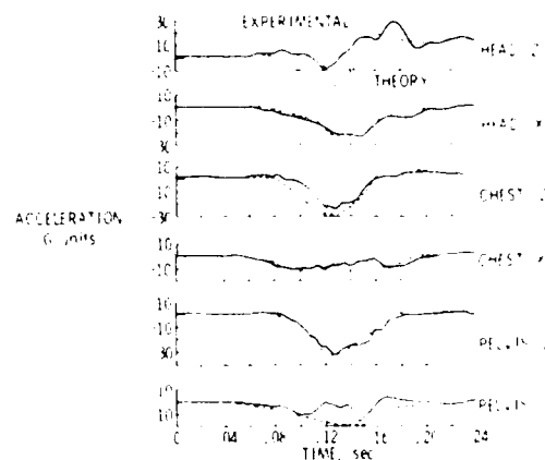
Fig. 9 Experimental and computer dummy accelerations for the -30 deg. 27 m/s full-scale crash test.
